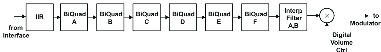
Figure 3-2. Signal Chain for PRB_P1 and PRB_P3
