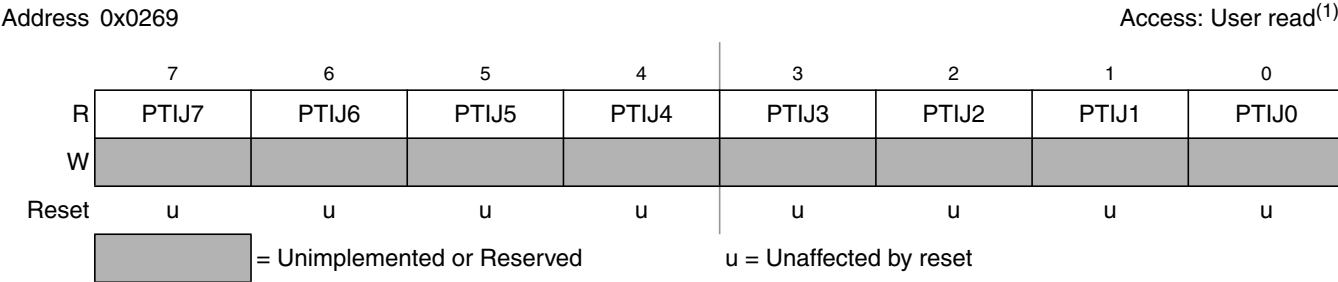
Figure 2-60. Port J Input Register (PTIJ)
