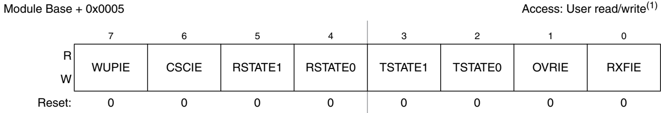
Figure 16-9. MSCAN Receiver Interrupt Enable Register (CANRIER)
