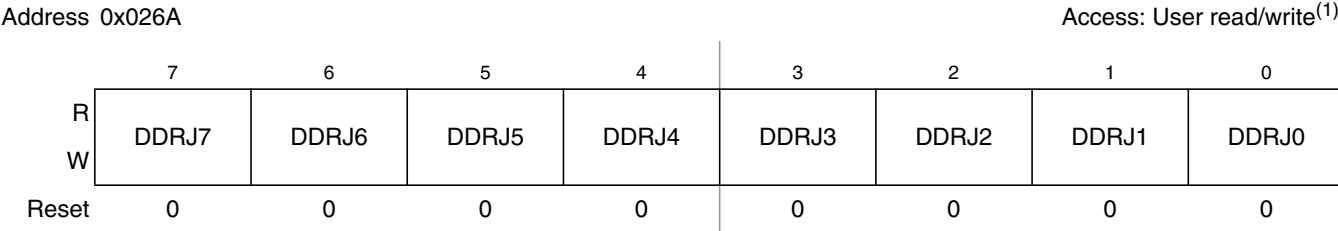
Figure 2-61. Port J Data Direction Register (DDRJ)
