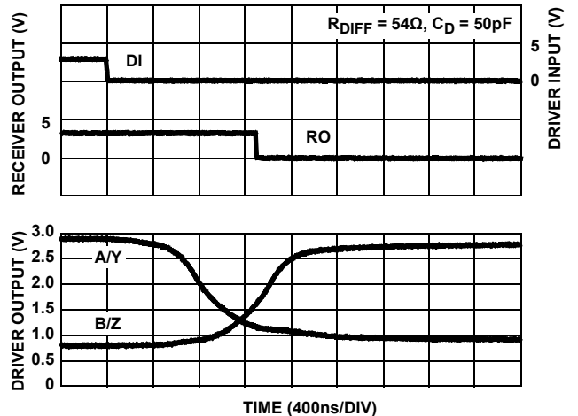
FIGURE 21. DRIVER AND RECEIVER WAVEFORMS, HIGH TO LOW (ISL3170E, ISL3171E, ISL3172E)
