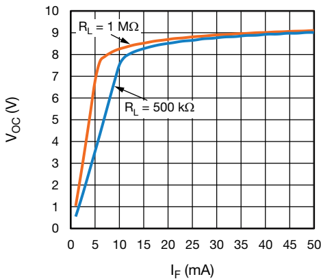
Fig. 2 - Output Open Circuit Voltage vs. LED Current
