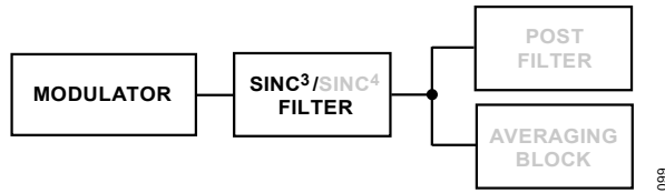
Figure 89. Sinc 3 Filter
