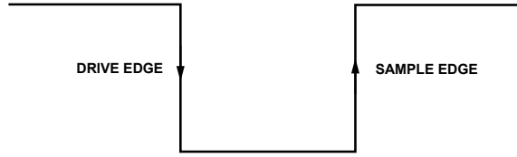
Figure 65. SPI Mode 3, SCLK Edges
