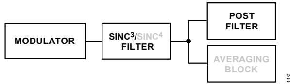
Figure 109. Post Filters
