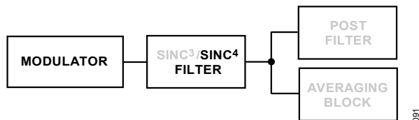
Figure 81. Sinc 4 Filter
