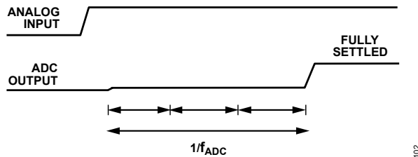
Figure 92. Sinc 3 Zero Latency Operation
