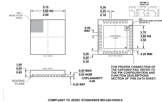
Figure 130. 32-Lead Lead Frame Chip Scale Package [LFCSP] 5 mm x 5 mm Body and 0.95 mm Package Height (CP-32-30) Dimensions shown in millimeters
