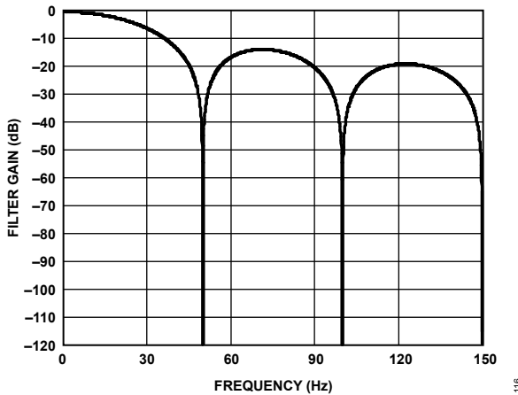
Figure 106. 50 Hz Rejection
