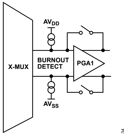
Figure 124. Burnout Currents
