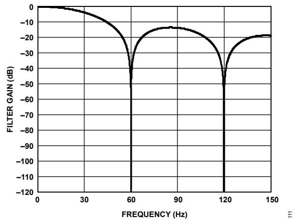
Figure 101. 60 Hz Rejection
