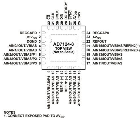
Figure 9. Pin Configuration
