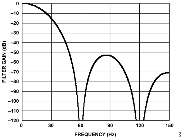
Figure 86. Sinc 4 Filter Response (60 SPS Output Data Rate, Zero Latency Disabled or 15 SPS Output Data Rate, Zero Latency Enabled)
