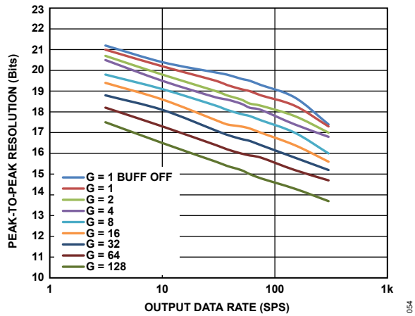
Figure 54. Peak-to-Peak Resolution vs. Output Data Rate, Sinc^4 + Sinc^1 Filter (Mid Power Mode)
