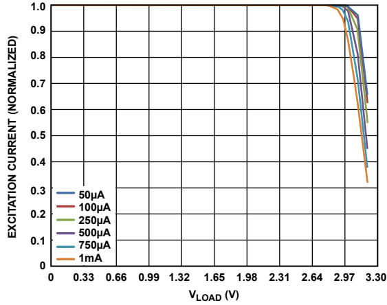
Figure 34. Output Compliance ( AV_{DD} = 3.3\text{ V} )
