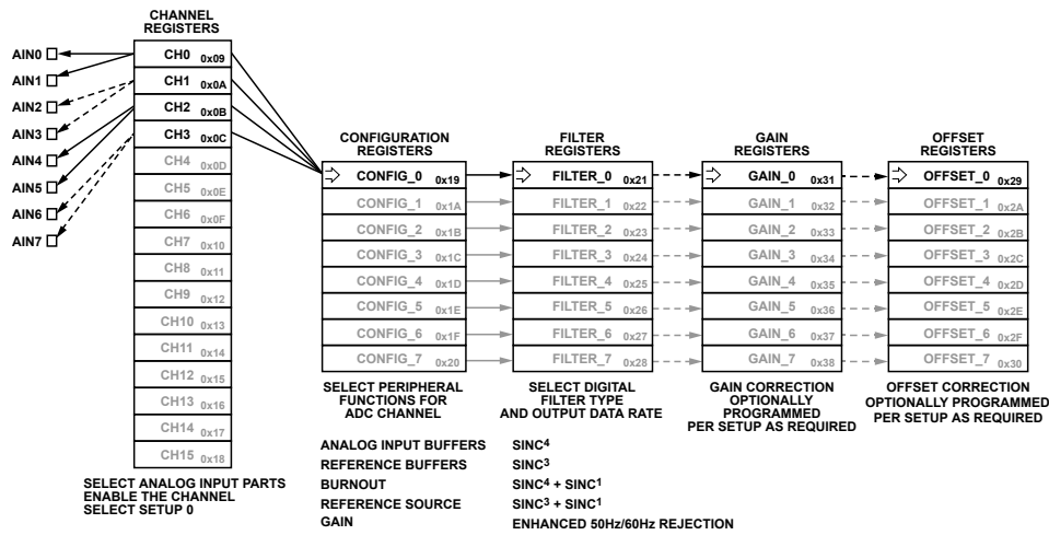
Figure 70. Four Fully Differential Inputs, All Using a Single Setup (CONFIG_0, FILTER_0, GAIN_0, OFFSET_0)
