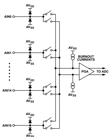
Figure 73. Analog Input Multiplexer Circuit
