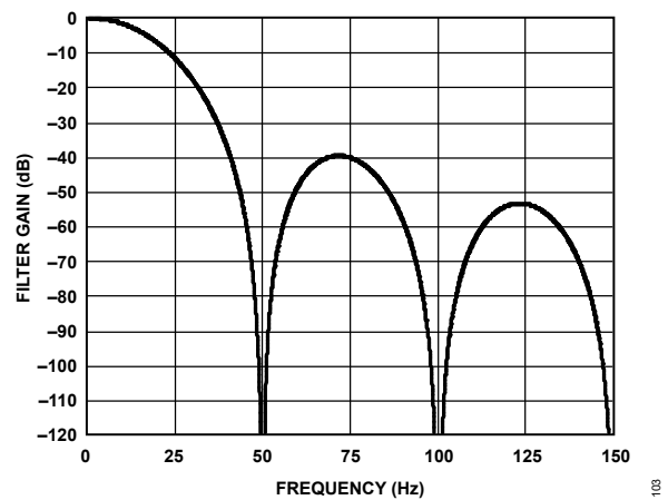
Figure 93. Sinc 3 Filter Response (50 SPS Output Data Rate, Zero Latency Disabled or 16.67 SPS Output Data Rate, Zero Latency Enabled)
