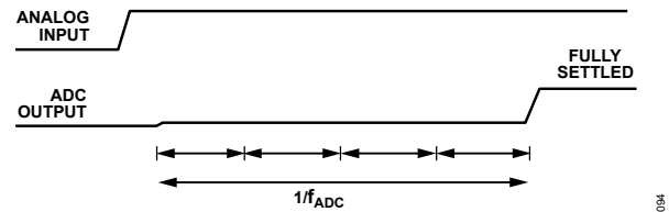
Figure 84. Sinc 4 Zero Latency Operation
