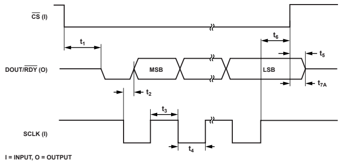
Figure 4. Read Cycle Timing Diagram ( \overline{CS\_EN} Bit Set)
