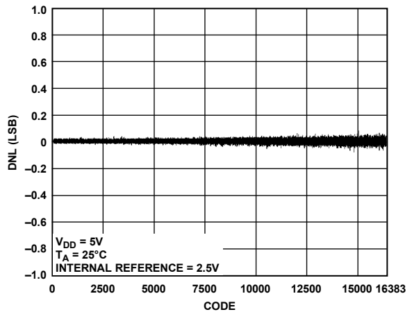
Figure 19. AD5685R DNL
