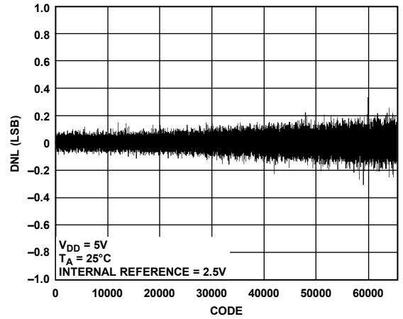
Figure 18. AD5686R DNL
