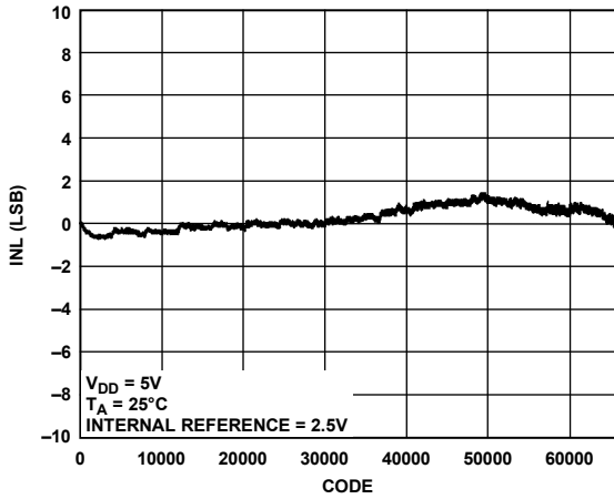
Figure 15. AD5686R INL
