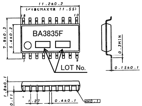
Outline Dimension
