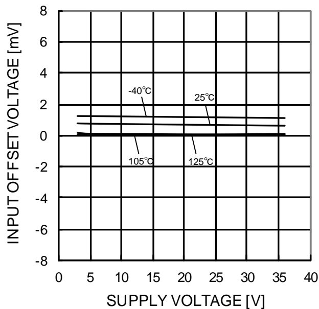
Figure 61. Input Offset Voltage - Supply Voltage (VICM=0V, OUT=1.4V)
