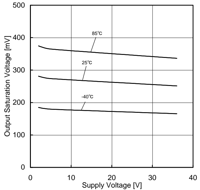
Figure 28. Output Saturation Voltage vs Supply Voltage (I OL =4mA)
