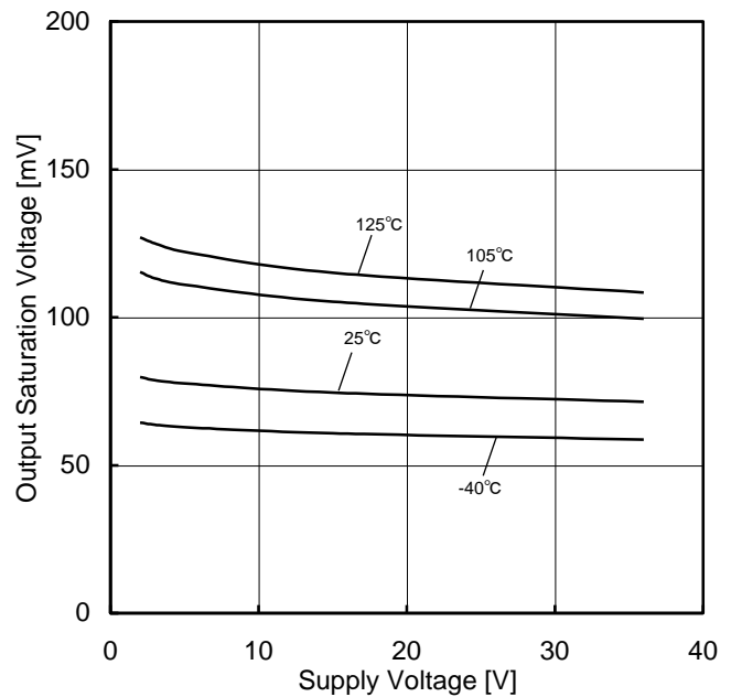
Figure 91. Output Saturation Voltage vs Supply Voltage (I OL =4mA)
