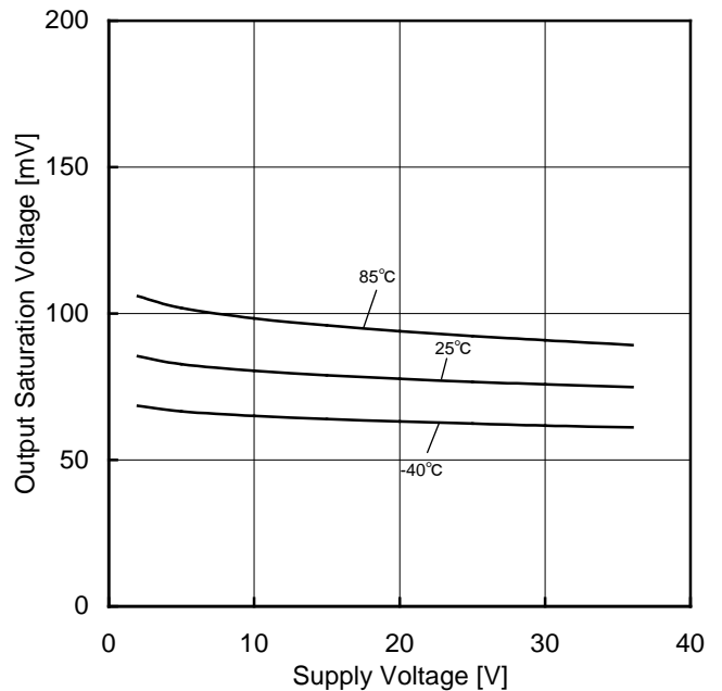
Figure 5. Output Saturation Voltage vs Supply Voltage (I OL =4mA)
