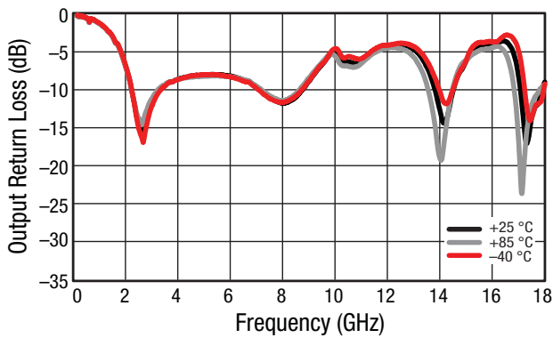
Figure 24. Small Signal Output Return Loss (S22) vs Frequency and Temperature, Wide Band
