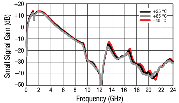
Figure 8. Small Signal Gain (IS21) vs Frequency and Temperature, Wide Band
