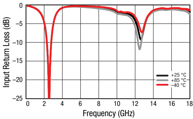
Figure 22. Small Signal Input Return Loss (S11) vs Frequency and Temperature, Wide Band
