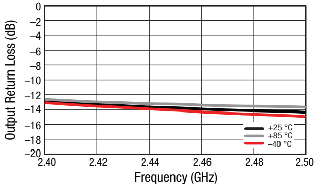
Figure 20. Small Signal Output Return Loss (S22) vs Frequency and Temperature, Narrow Band
