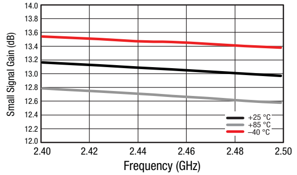
Figure 4. Small Signal Gain (IS21) vs Frequency and Temperature, Narrow Band
