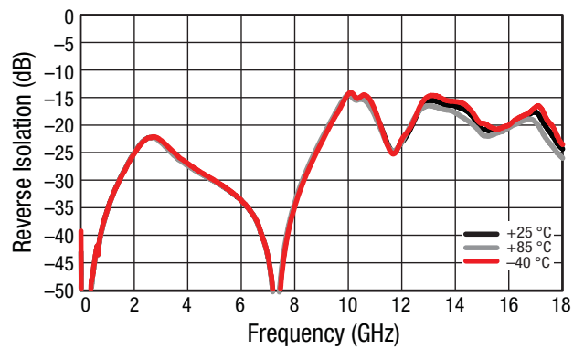
Figure 23. Small Signal Reverse Isolation (S12) vs Frequency and Temperature, Wide Band
