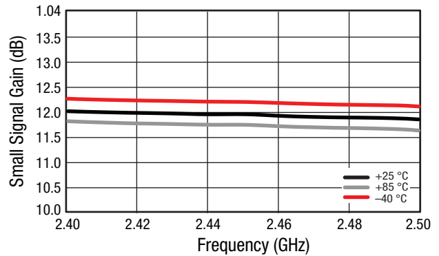
Figure 17. Small Signal Gain (IS21) vs Frequency and Temperature, Narrow Band
