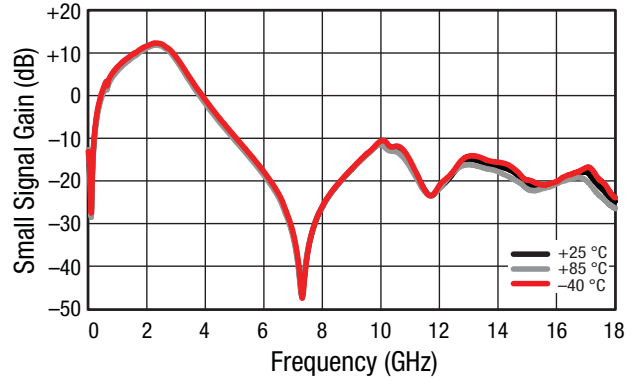
Figure 21. Small Signal Gain (S21) vs Frequency and Temperature, Wide Band
