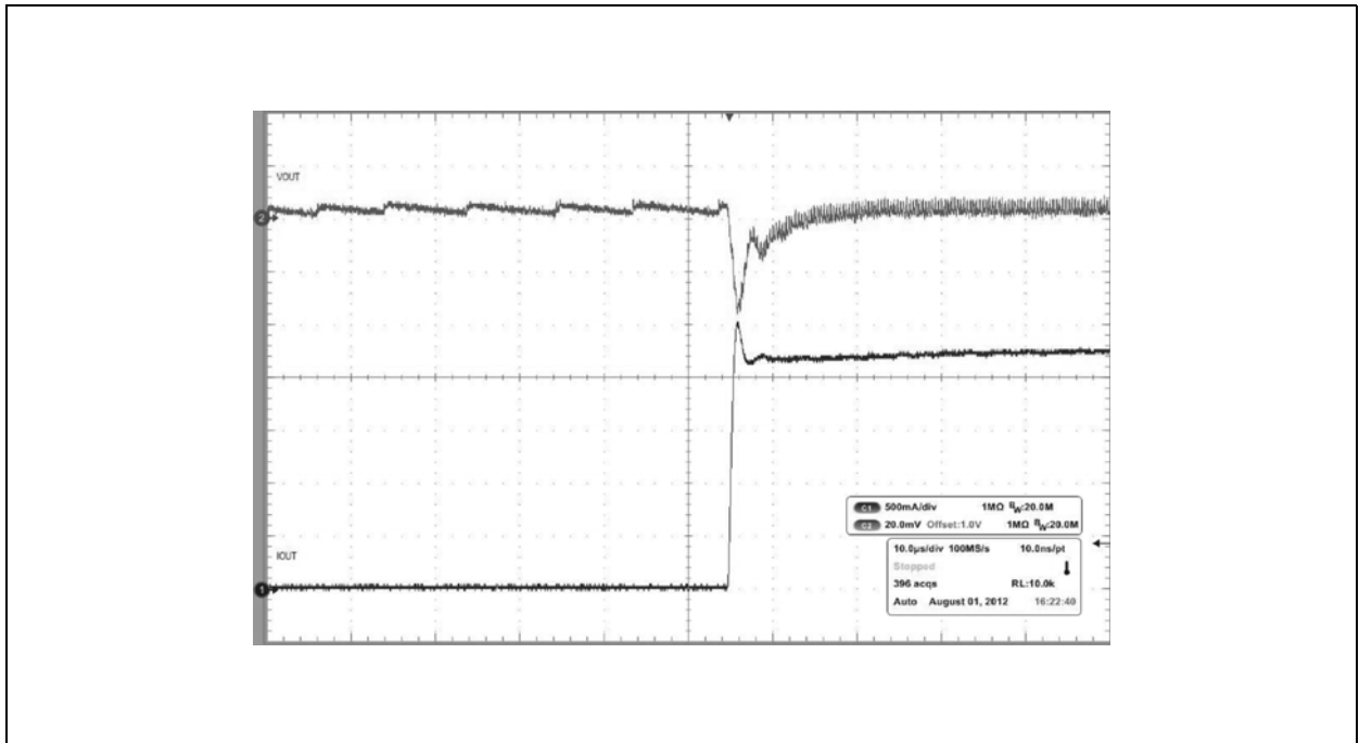
DC/DC Buck SD4 Low Noise Load Transient: Shows the response of the SD0 buck controller to a load transient from 0 to 2.3A @ 1.2V with VSUP=3.7V, 3MHz operation, fast=0, COUT=44µF, low_noise=1 and TA=25°C.
