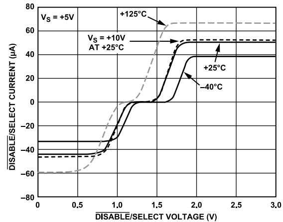
Figure 55. DISABLE/SELECT Current vs. DISABLE/SELECT Voltage and Temperature
