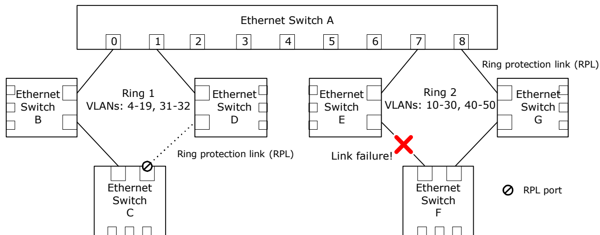
Figure 89 • Ethernet Ring with Failure
