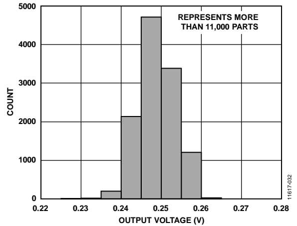
Figure 33. Output Voltage ( V_{OUT} ) Distribution, P_{IN} = -9 dBm at 12 GHz, 25°C
