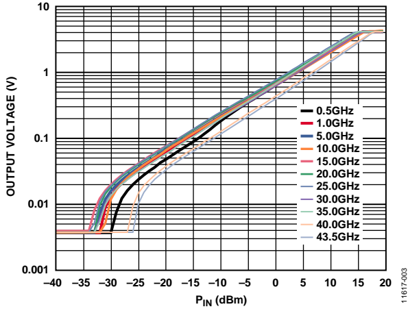
Figure 4. Typical Output Voltage ( V_{OUT} ) vs. RF Input Power ( P_{IN} ) at Various Frequencies (0.5 GHz to 43.5 GHz) at 25°C
