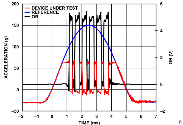
Figure 26. ADXL1001/ADXL1002 Behavior During a Continuous Overrange
