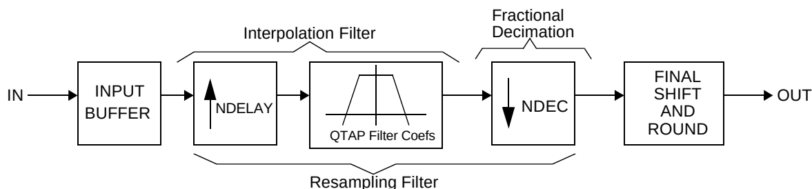
Figure 12. Resampler Channel Block Diagram
