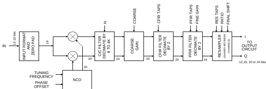
Figure 4. The Down Converter Channel
