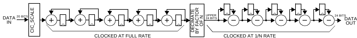
Figure 9. Five Stage CIC Decimate by N Filter
