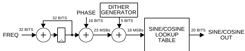
Figure 6. NCO Circuit
