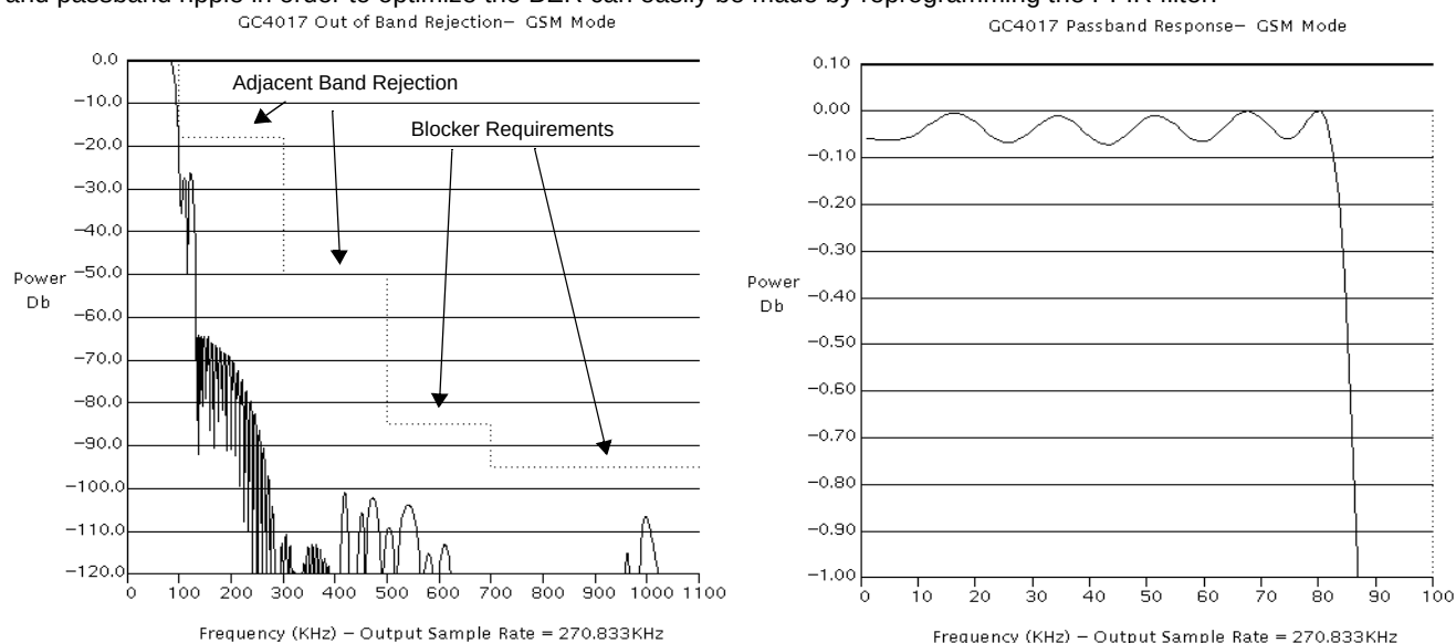
Figure 20. Frequency Response for the Example GSM Application
