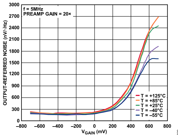
Figure 29. Output-Referred Noise vs. V_{GAIN} at Various Temperatures ( T ) When the Preamplifier Gain is 20× (See Figure 62)
