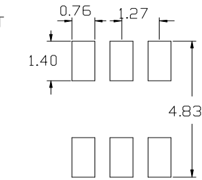
FOOTPRINT FOR PCB DESIGN
