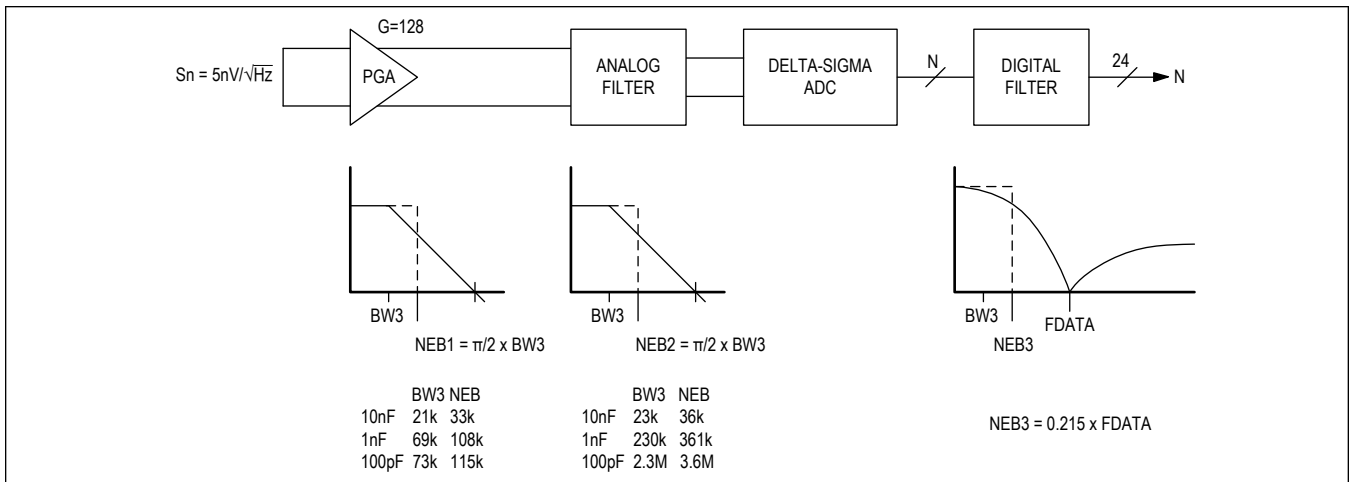
Figure 18. Signal Path Block Diagram Including Bandwidth of Each Stage
