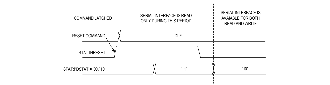
Figure 13. STAT:INRESET and STAT:PDSTAT Timing
