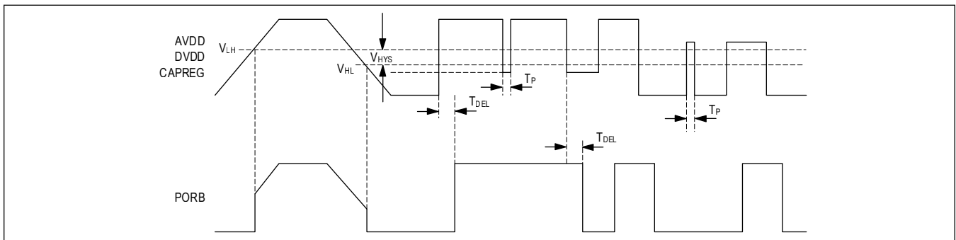
Figure 10. Undervoltage Lockout Characteristic Voltage Levels and Timing
