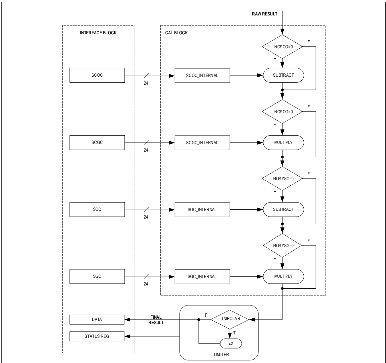
Figure 14. Calibration Flow Diagram
