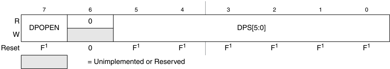
Figure 26-15. EEPROM Protection Register (EPPROT)
