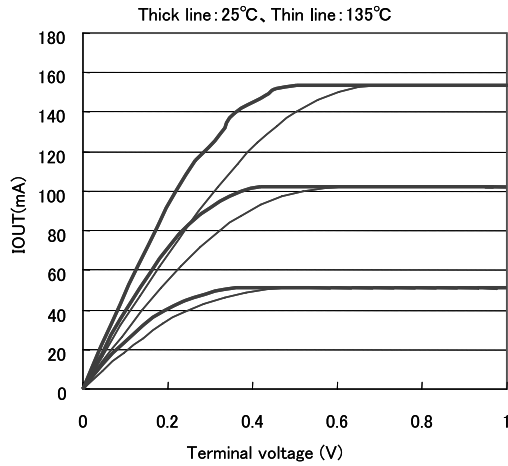
Fig.9 IOU(G) vs. Terminal voltage
