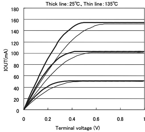
Fig.8 IOU(T) vs. Terminal voltage
