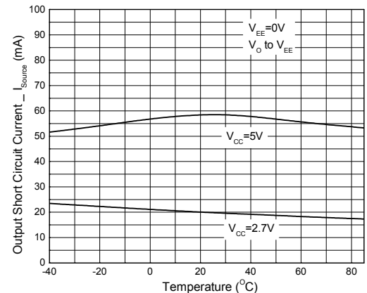
Output Short Circuit Current vs. Temperature
