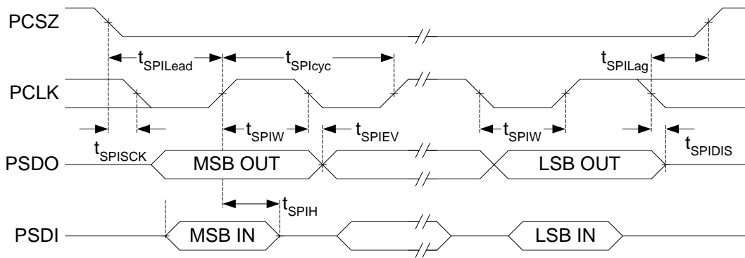
Figure 5: SPI Slave Port (MISSION Mode) Timing
