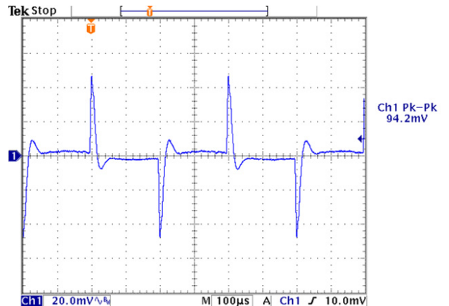
Figure 20. Transient Response without Optimal Voltage Positioning
