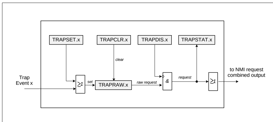
Figure 11-4 Trap Subsystem
