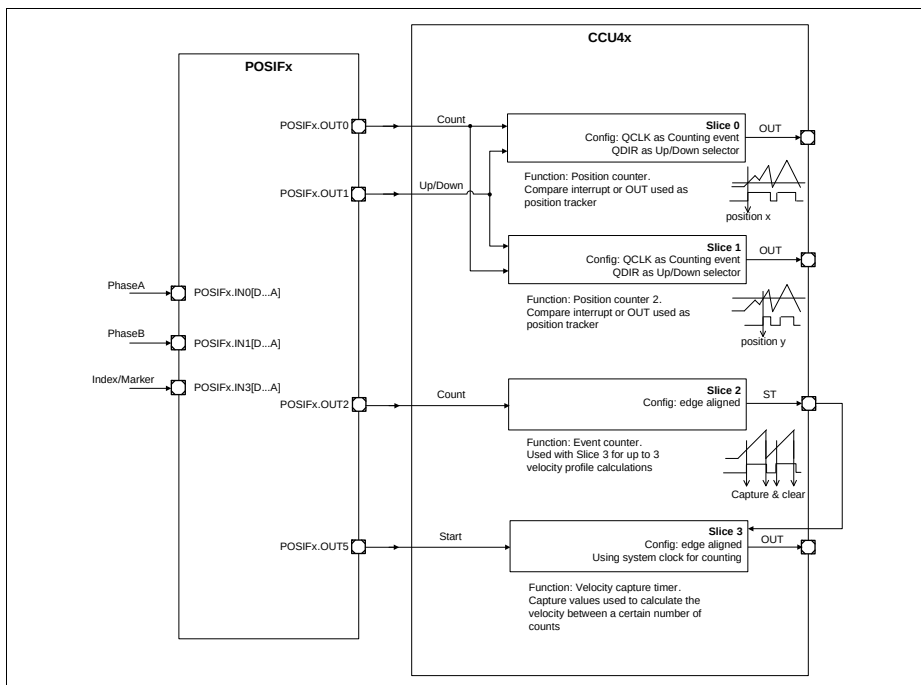
Figure 24-18 Quadrature Decoder Mode usage - profile 2
