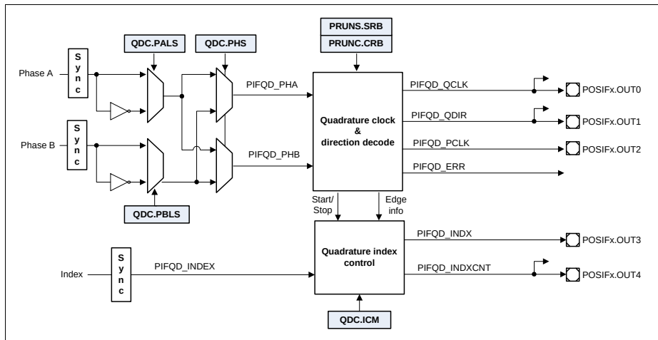
Figure 24-9 Quadrature Decoder Control Overview
