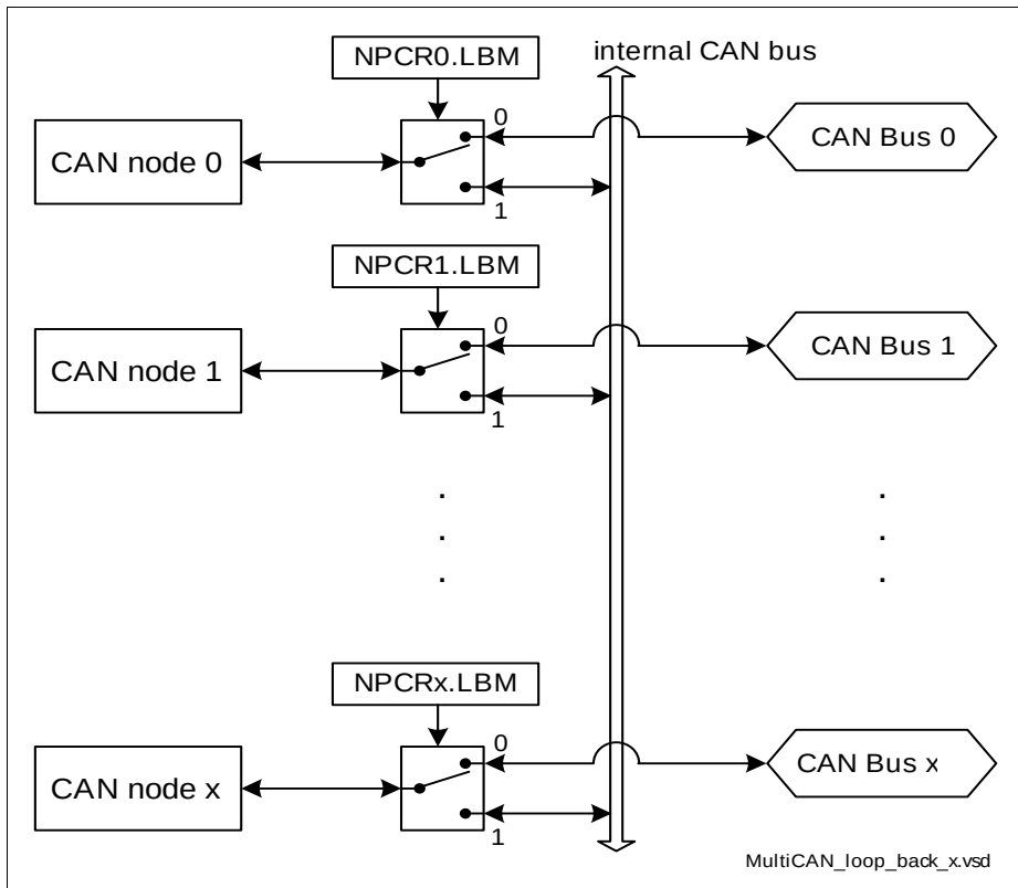
Figure 18-12 Loop-Back Mode
