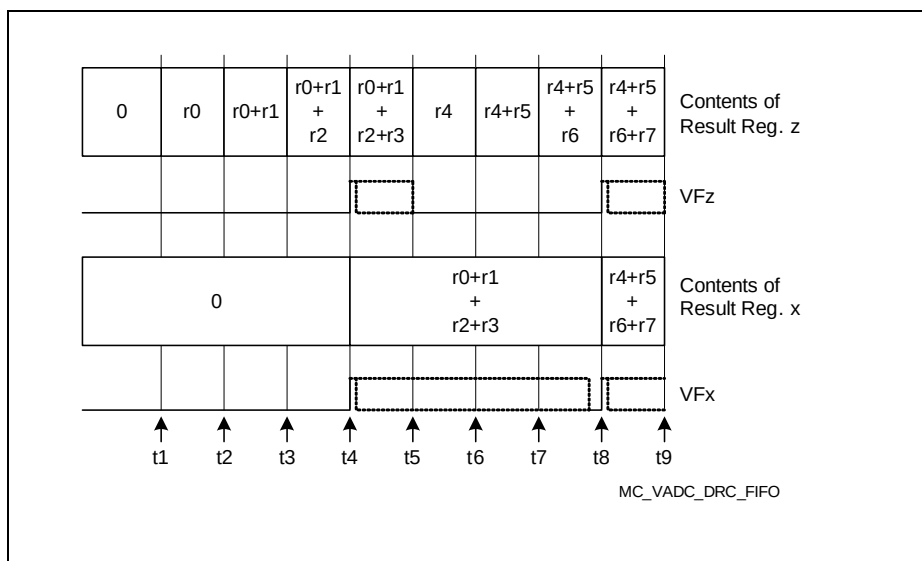
Figure 19-19 Standard Data Reduction Filter with FIFO Enabled
