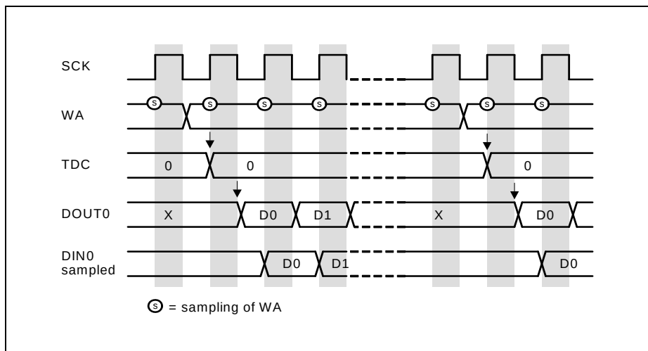
Figure 17-61 Transfer Delay with Delay 1
