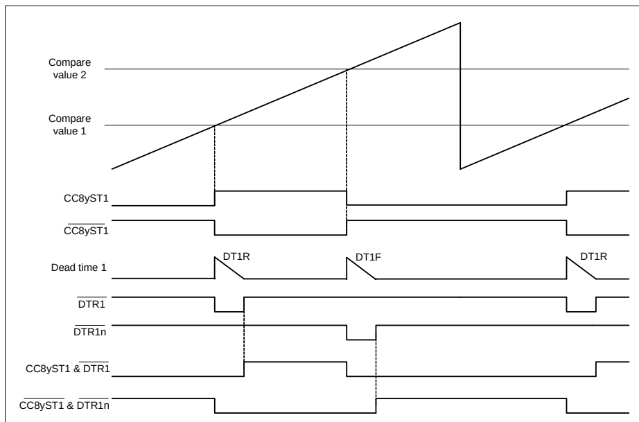
Figure 23-24 Edge Aligned - Asymmetric PWM timing, CC8yCR1.CR1 < CC8yCR2.CR2
