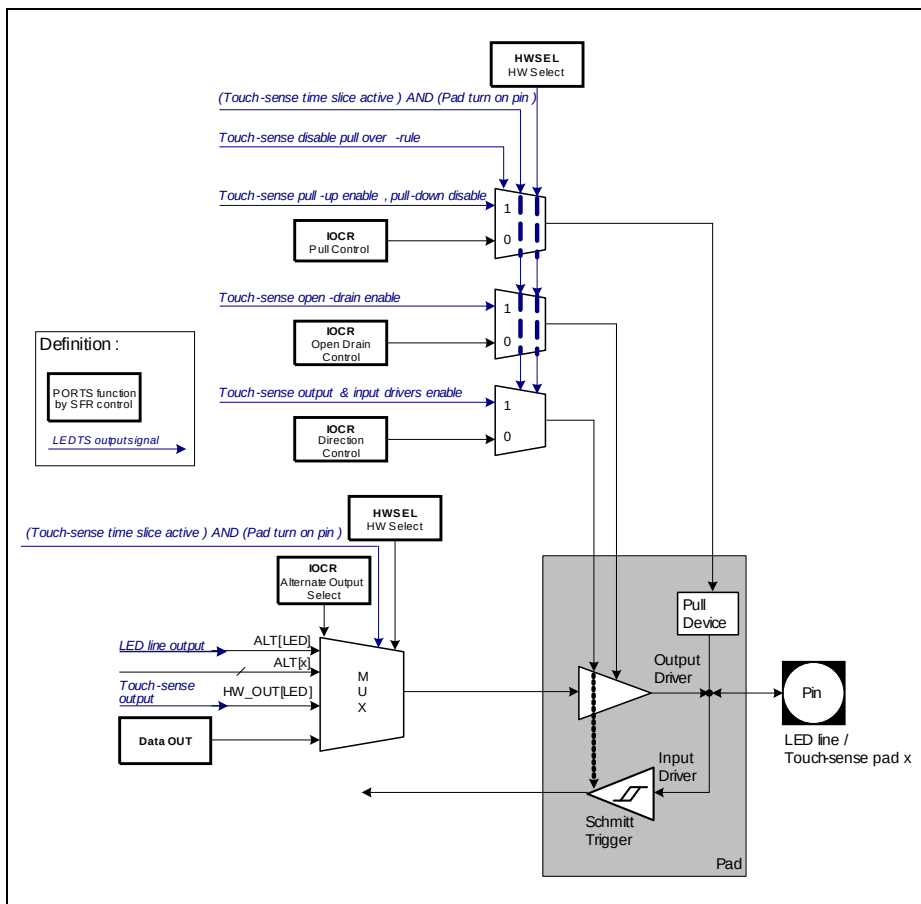
Figure 12-8 Over-rule Control on Pin for Touch-Sense Function
