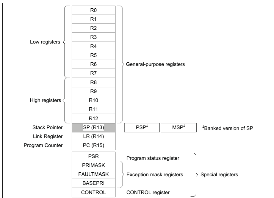
Figure 2-2 Core registers
