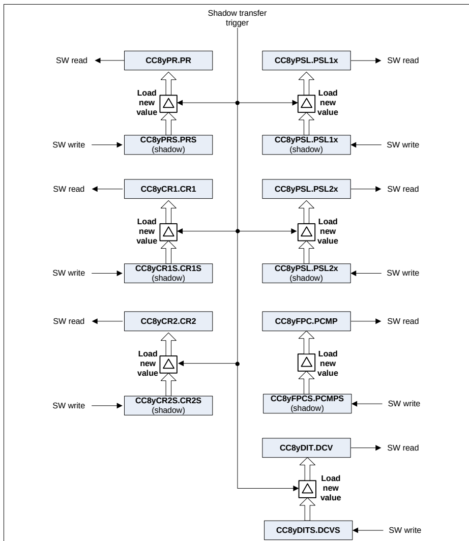
Figure 23-8 Shadow registers overview
