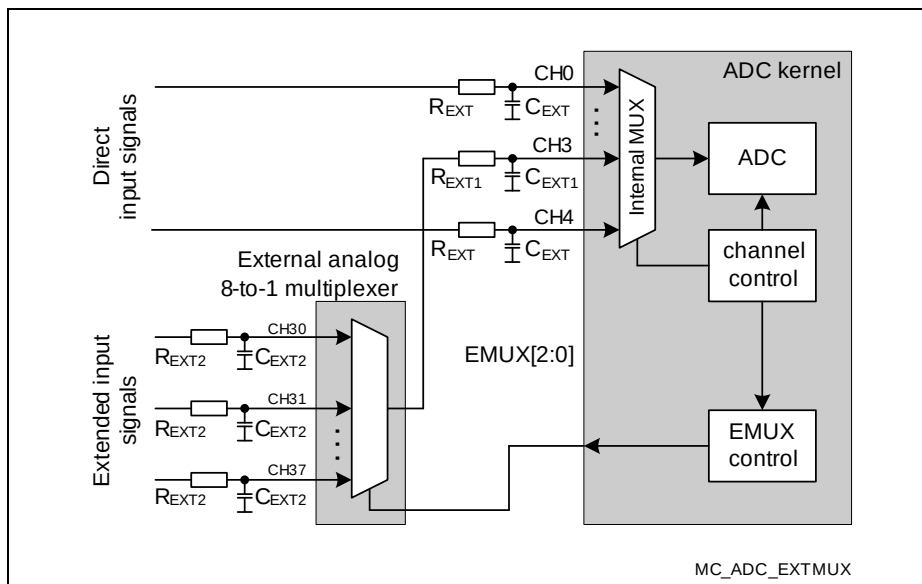
Figure 19-28 External Analog Multiplexer Example
