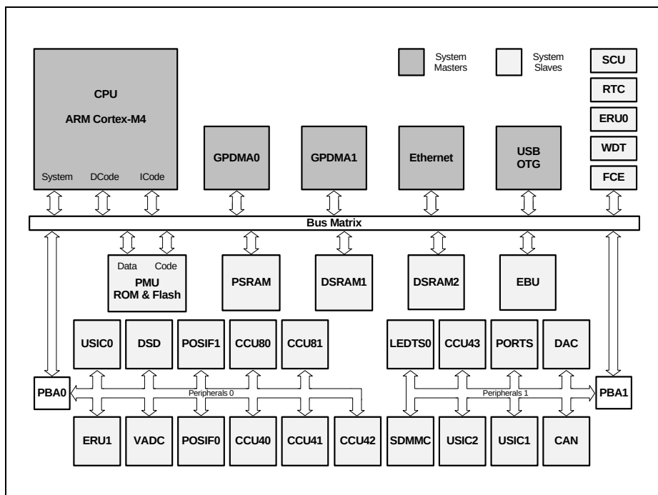
Figure 1-1 XMC4500 System
