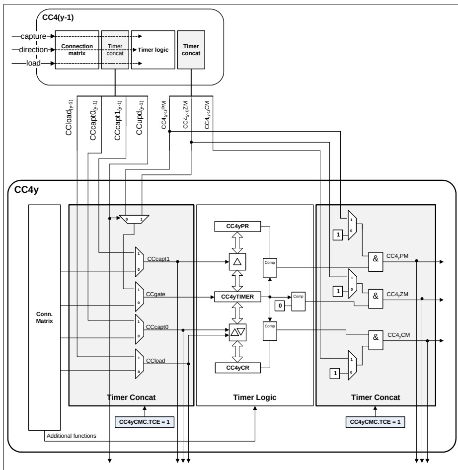
Figure 22-44 Timer concatenation control logic
