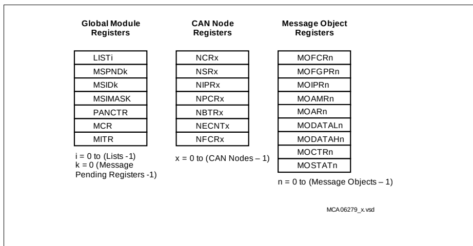
Figure 18-24 MultiCAN Kernel Registers
