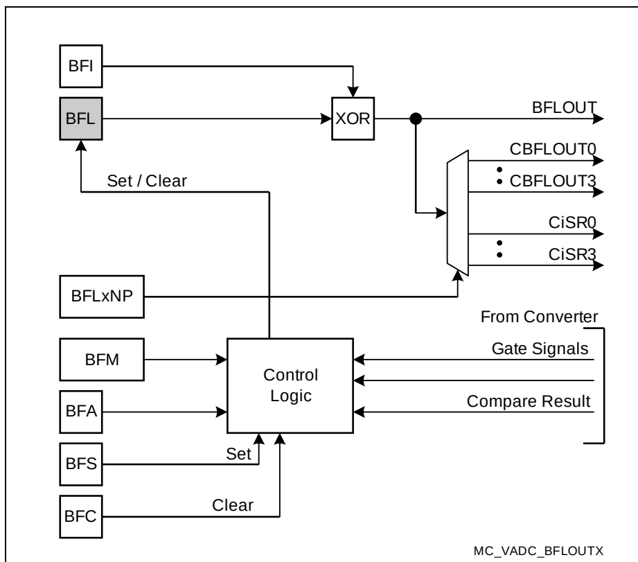
Figure 19-14 Boundary Flag Control
