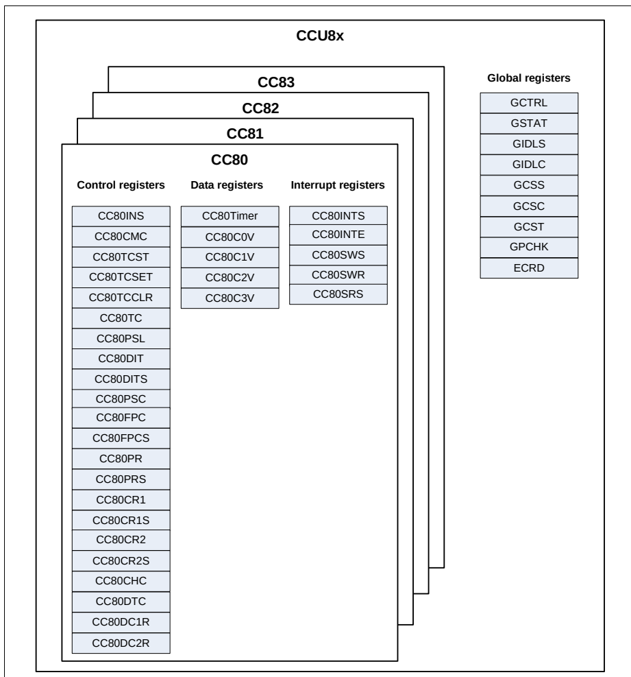
Figure 23-90 CCU8 registers overview
