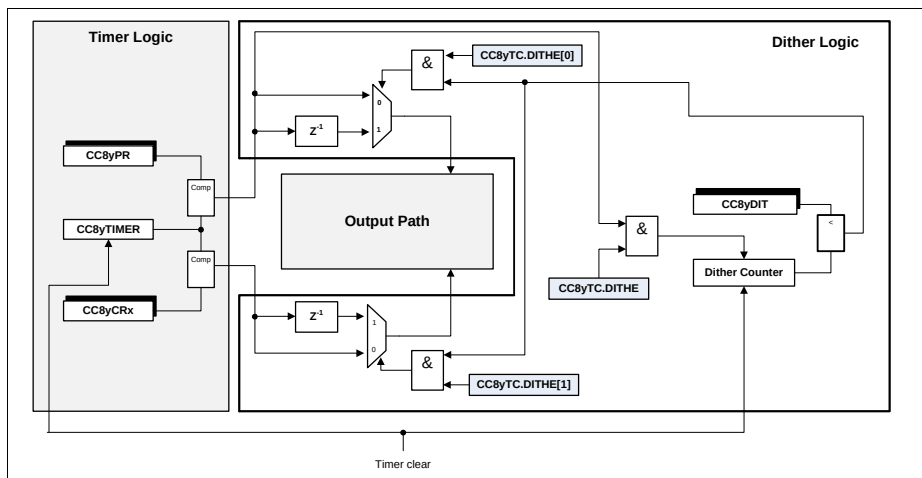
Figure 23-64 Dither control logic
