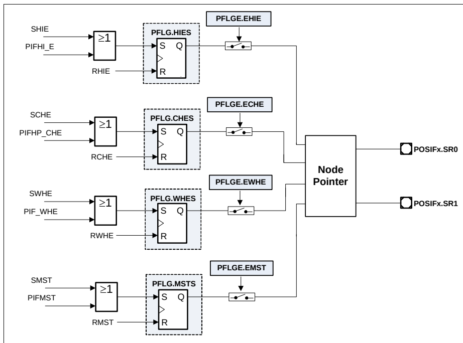
Figure 24-23 Hall Sensor Mode flags
