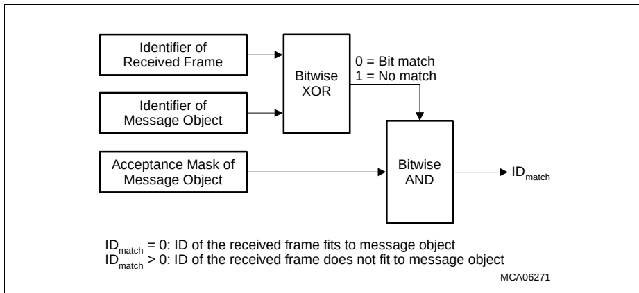
Figure 18-13 Received Message Identifier Acceptance Check
