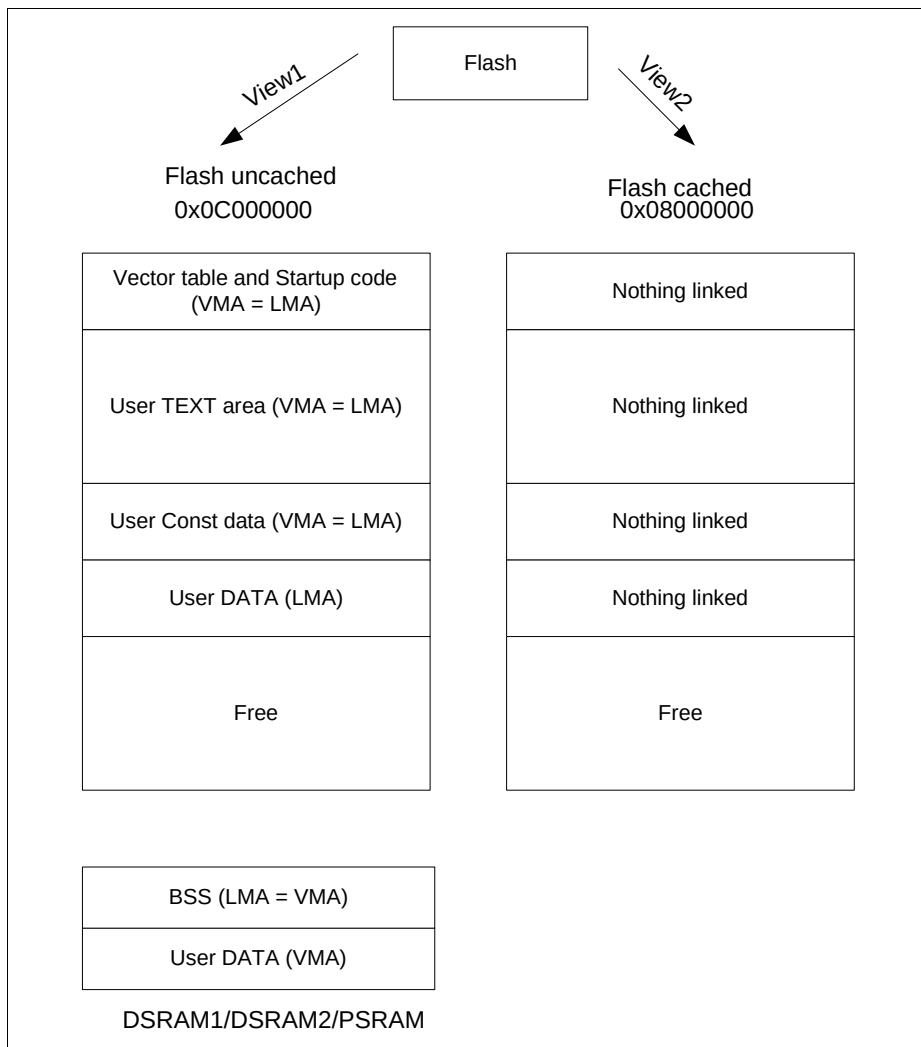
Figure 26-4 Memory Layout1
