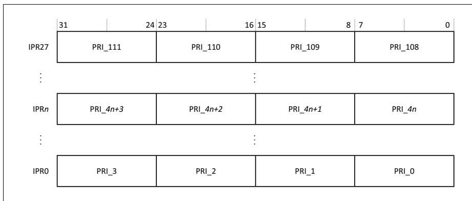
Figure 2-10 Interrupt Priority Register
