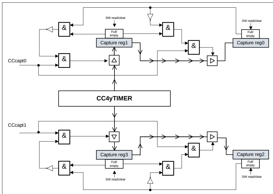
Figure 22-26 Slice capture logic
