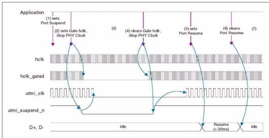
Figure 16-67 Host Mode Suspend and Resume With Clock Gating
