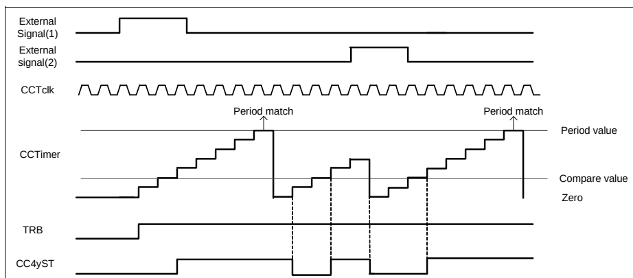
Figure 22-17 Start (as start)/ stop (as flush) - CC4yTC.STRM = 0_B , CC4yTC.ENDM = 01_B
