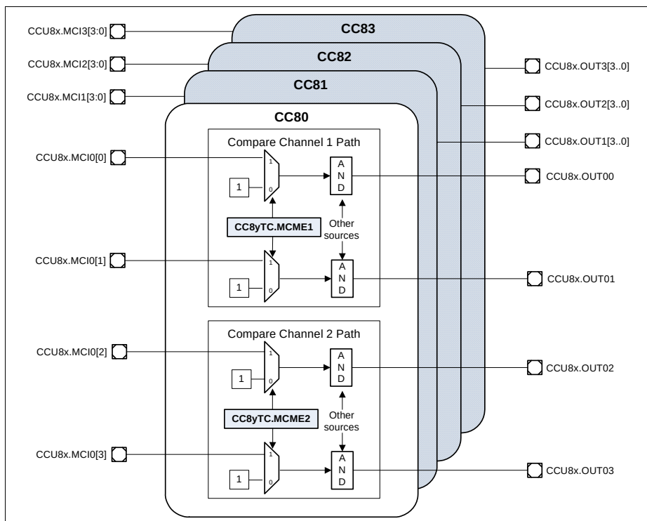
Figure 23-52 CCU8 Multi Channel overview
