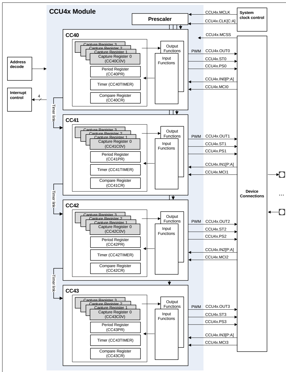
Figure 22-1 CCU4 block diagram
