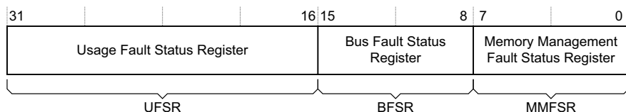
Figure 2-9 CFSR
