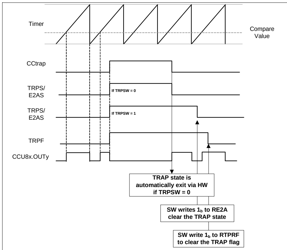
Figure 23-48 Trap timing diagram, CC8yTCST.CDIR = 0 CC8yPSL.PSL = 0
