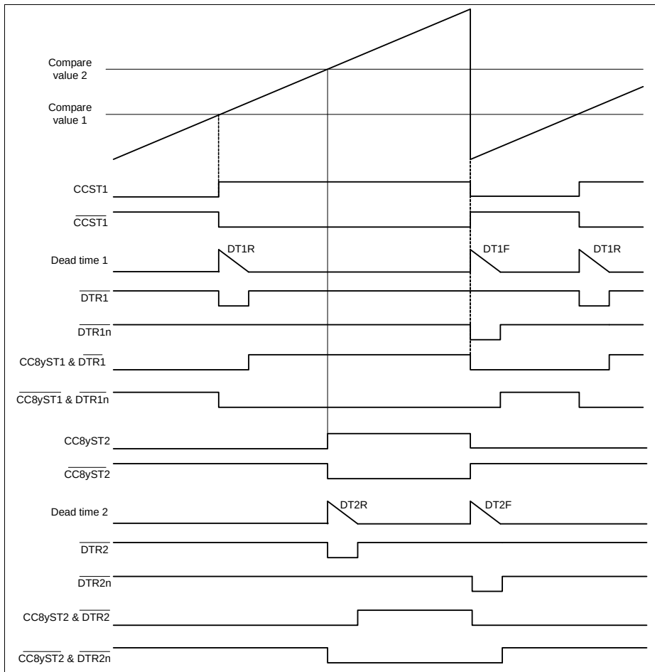
Figure 23-22 Edge Aligned - four outputs with dead time
