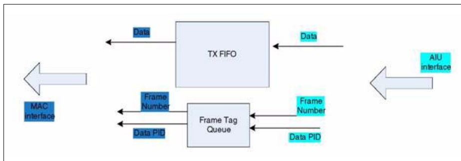
Figure 16-58 ISO IN Data Flow
