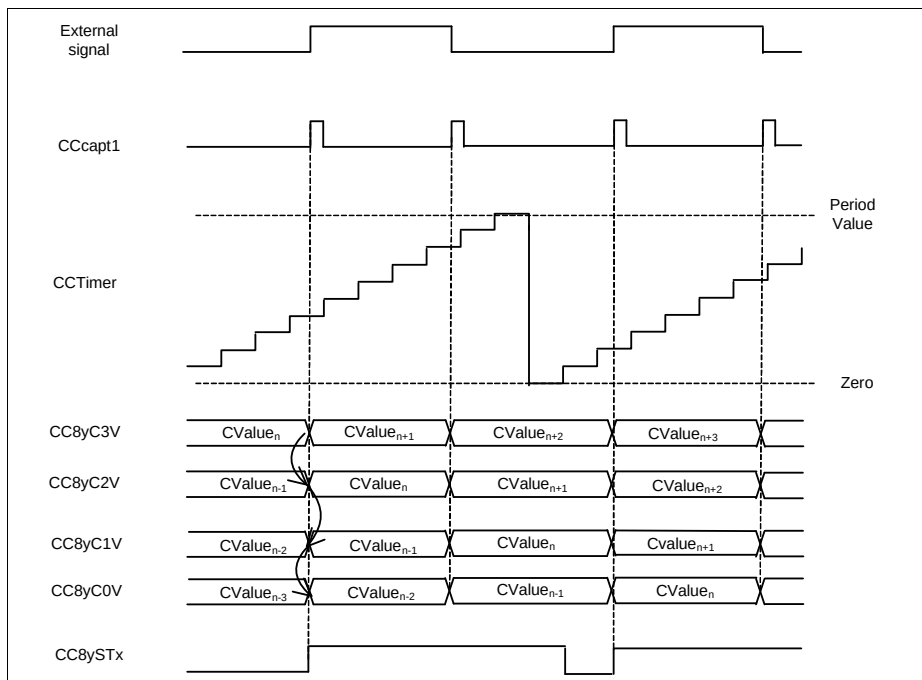
Figure 23-42 External Capture - \text{CC8yTC.SCE} = 1_{\text{B}}
