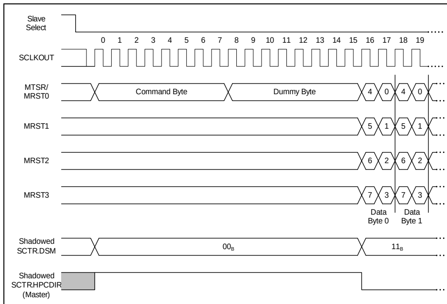
Figure 17-42 Quad-SSC Example
