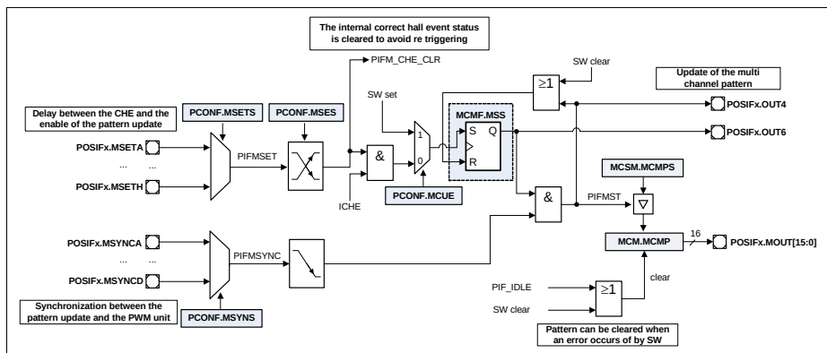
Figure 24-6 Multi-Channel Mode Diagram
