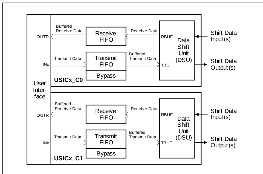
Figure 17-20 FIFO Buffer Overview
