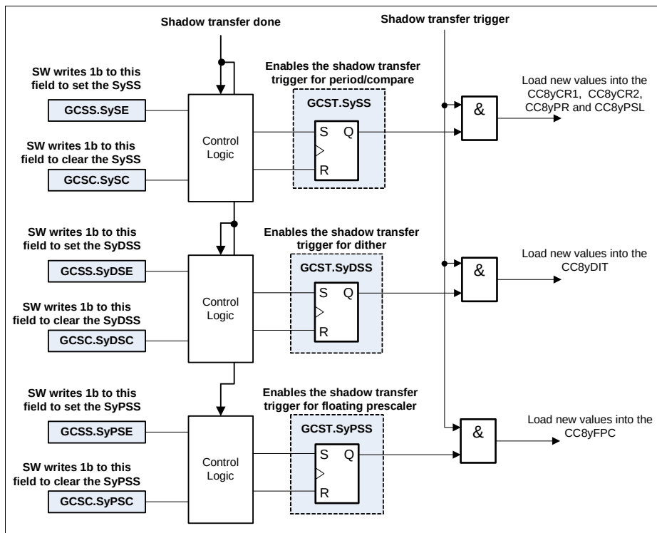
Figure 23-9 Shadow transfer enable logic
