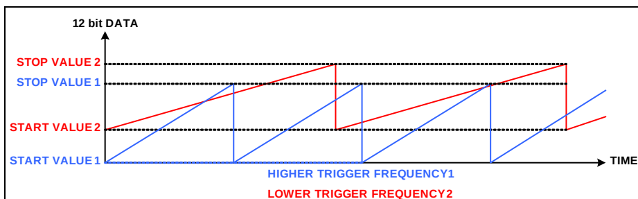
Figure 21-11 Unsigned 12-bit Ramp Generator Example Output
