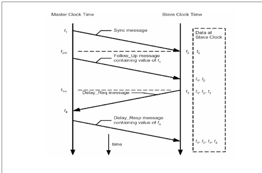
Figure 15-26 Networked Time Synchronization
