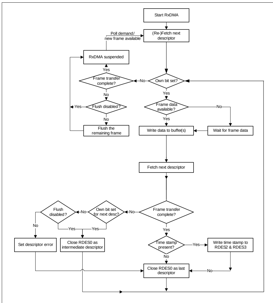
Figure 15-5 Receive DMA Operation
