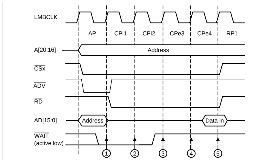
Figure 14-19 External Wait Insertion (Asynchronous Mode)
