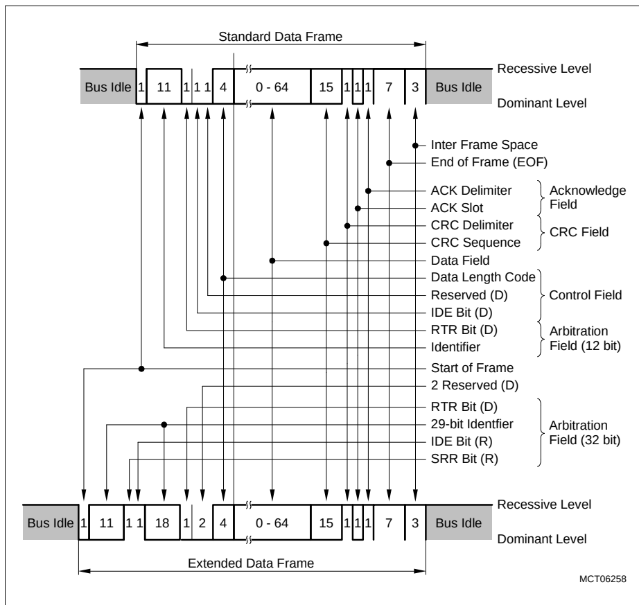
Figure 18-2 CAN Data Frame
