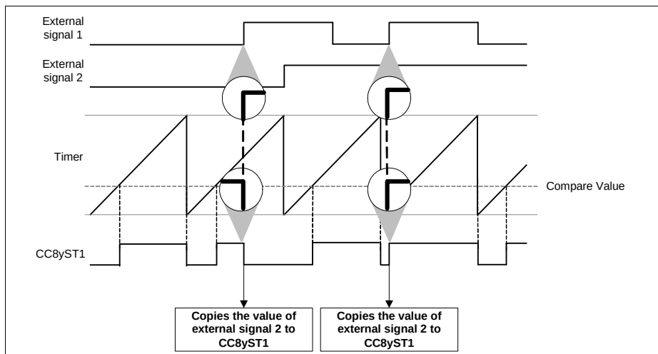
Figure 23-50 Status bit override
