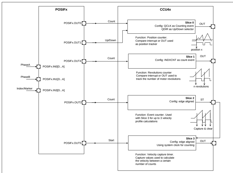
Figure 24-17 Quadrature Decoder Mode usage - profile 1
