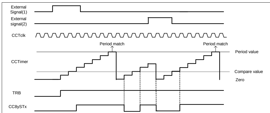
Figure 23-31 Start (as start)/ stop (as flush) - CC8yTC.STRM = 0_B , CC8yTC.ENDM = 01_B
