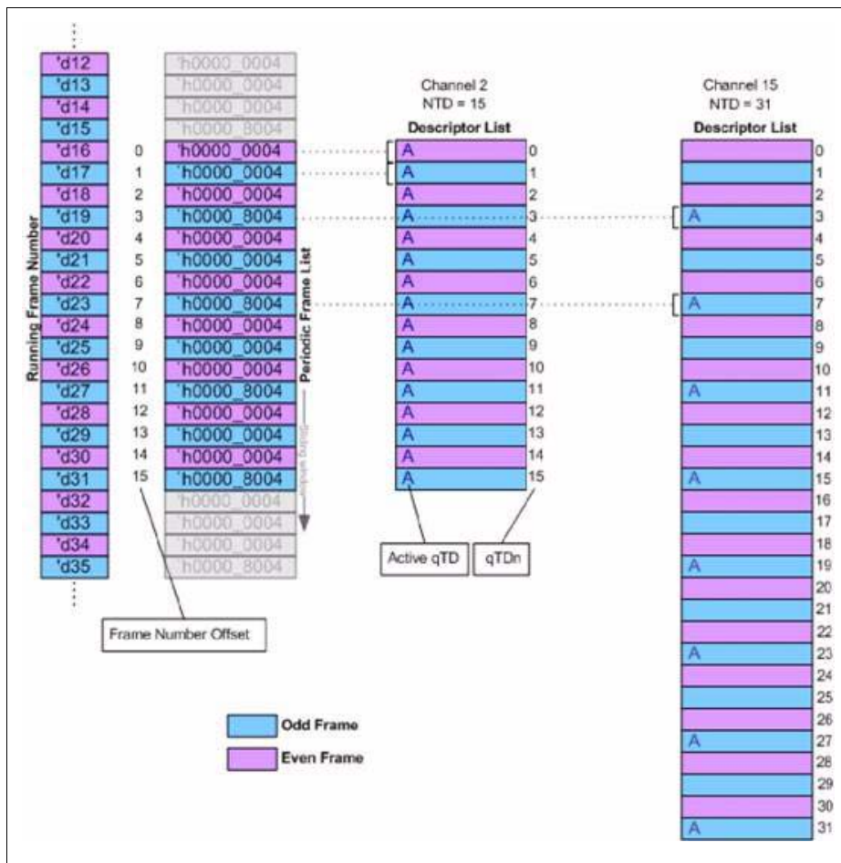
Figure 16-21 Full Speed Isochronous Transfer Scheduling
