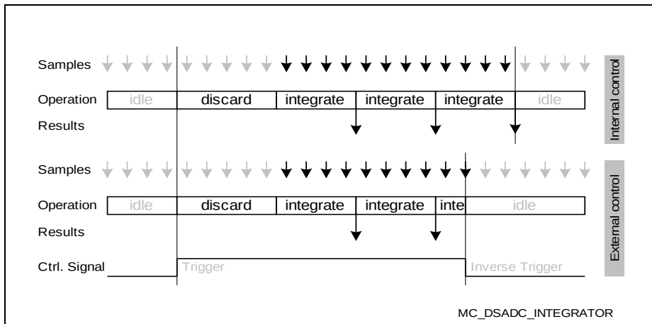
Figure 20-8 Integrator Operation
