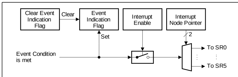
Figure 17-6 General Event and Interrupt Structure
