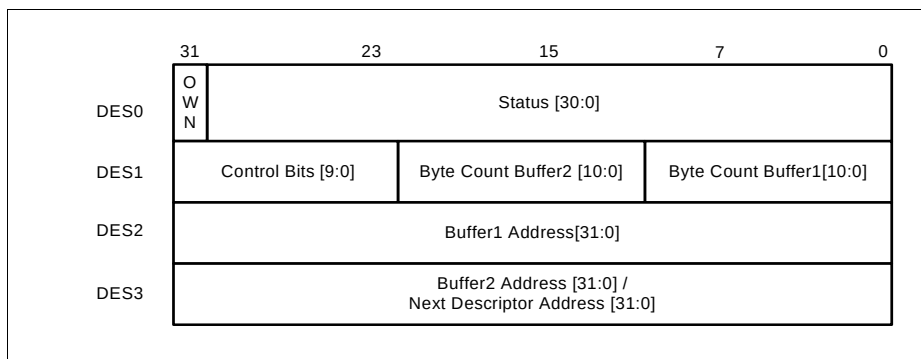
Figure 15-6 Rx/Tx Descriptors
