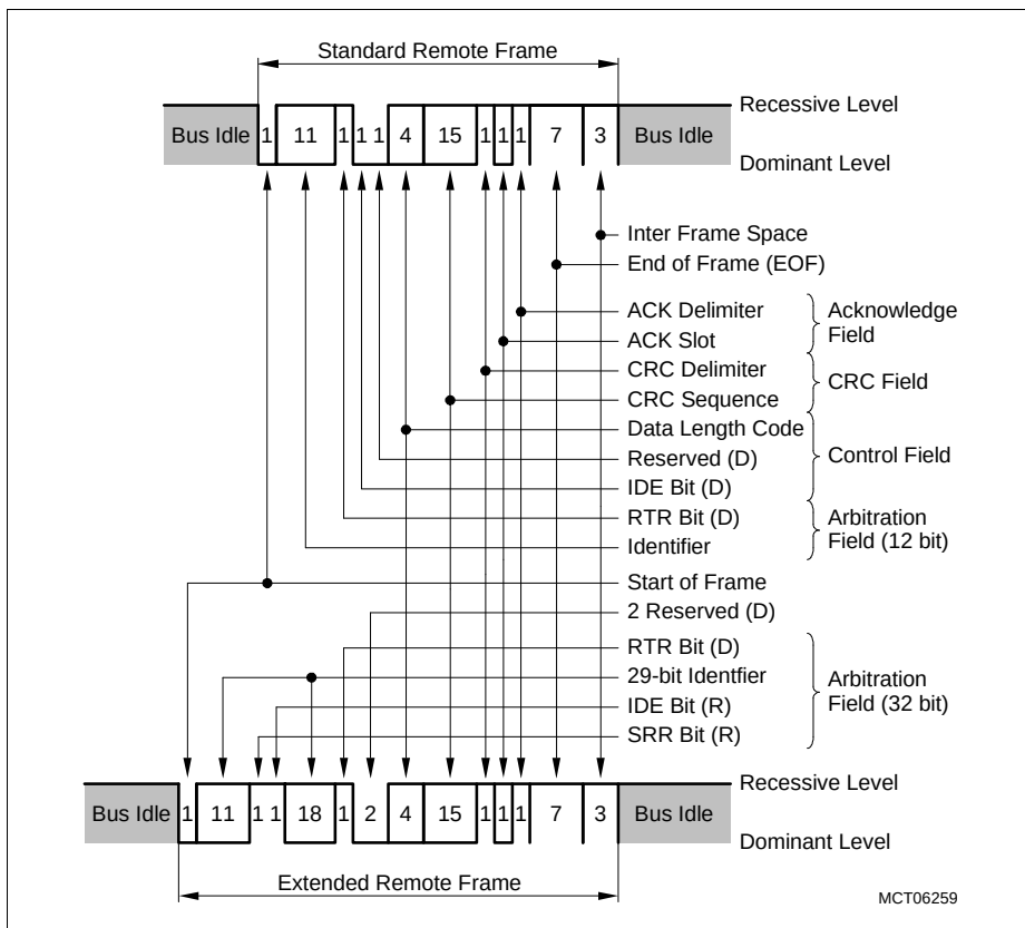
Figure 18-3 CAN Remote Frame
