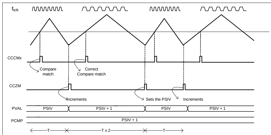
Figure 23-79 Floating Prescaler compare mode usage - Center Aligned
