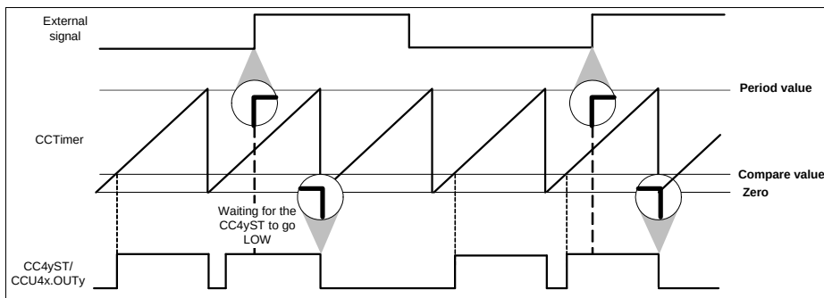
Figure 22-30 External modulation clearing the ST bit - \text{CC4yTC.EMT} = 0_B , \text{CC4yTC.EMS} = 1_B
