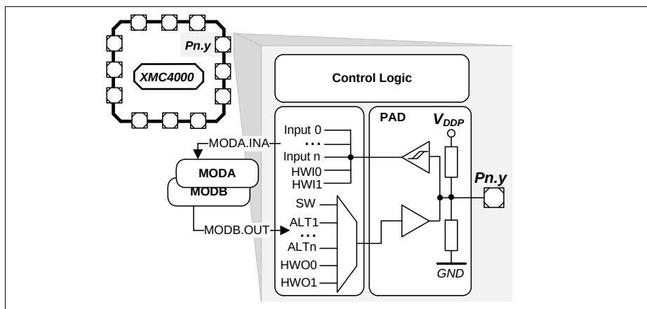
Figure 25-4 Simplified Port Structure
