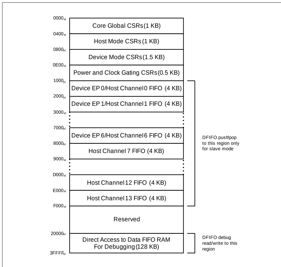
Figure 16-73 CSR Memory Map
