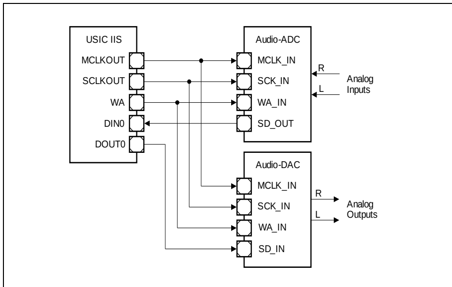
Figure 17-60 Connection of External Audio Devices
