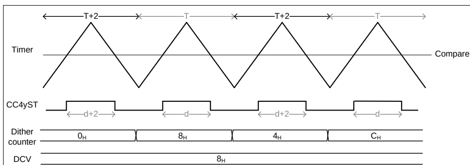
Figure 22-50 Dither timing diagram in center aligned - \text{CC4yTC.DITHE} = 01_B
