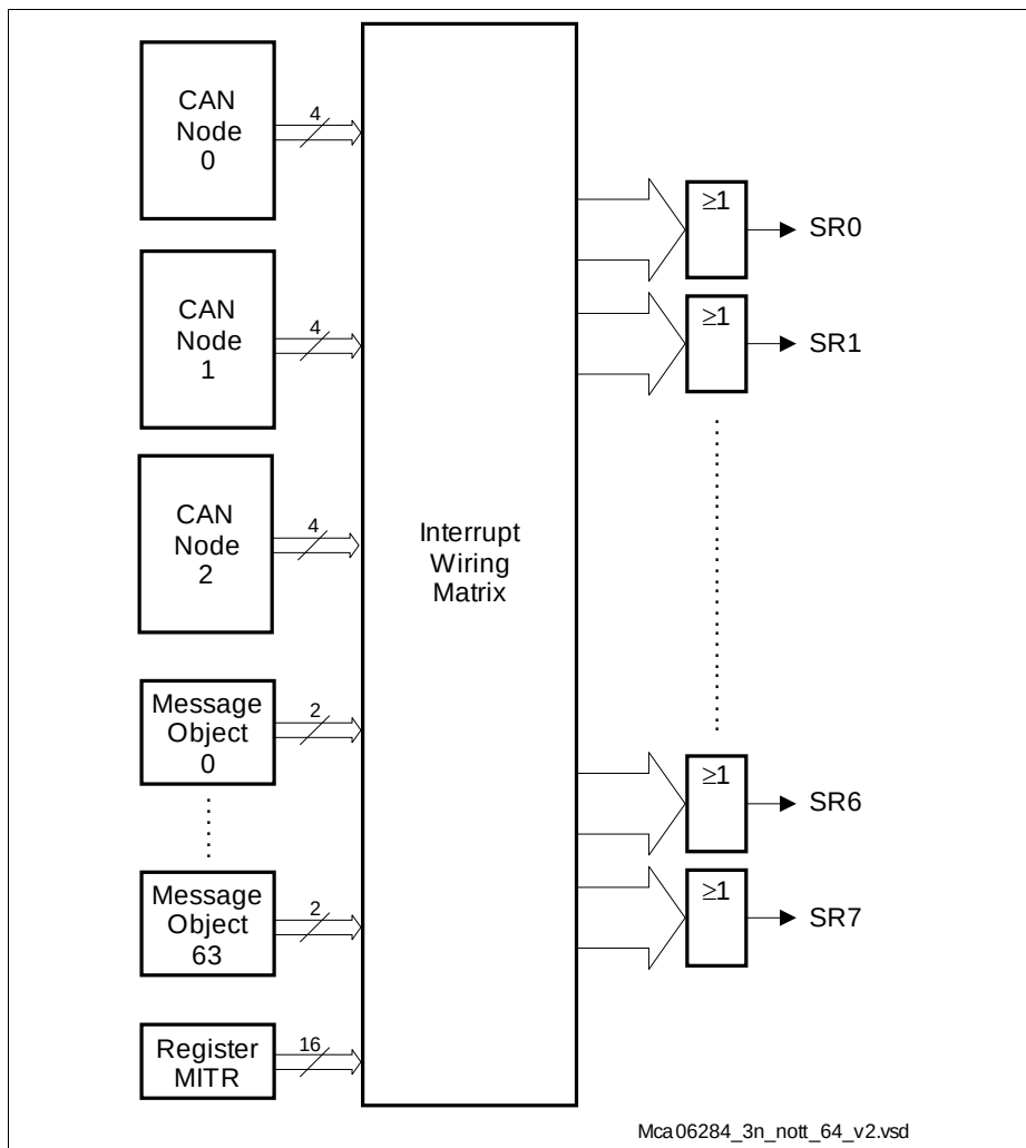
Figure 18-21 Interrupt Compressor
