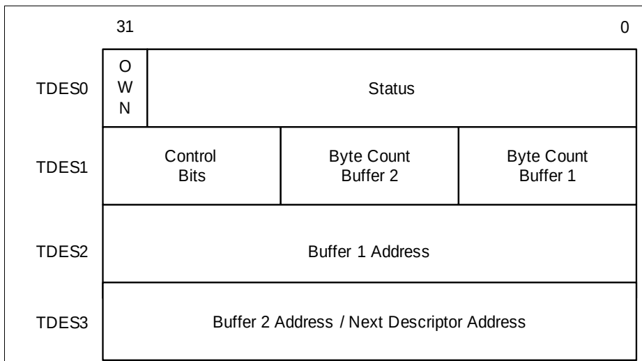
Figure 15-8 Transmit Descriptor Format
