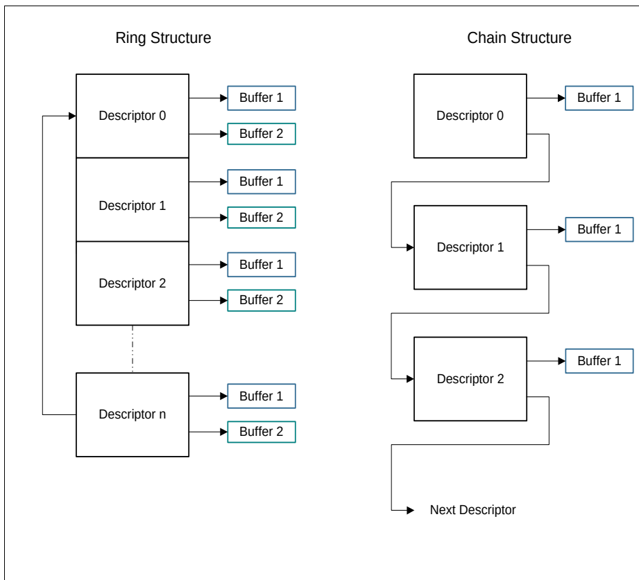
Figure 15-2 Descriptor Ring and Chain Structure
