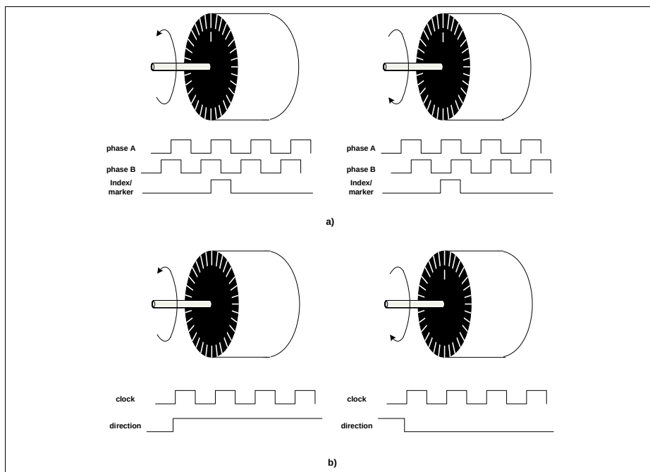
Figure 24-8 Rotary encoder types - a) standard two phase plus index signal; b) clock plus direction
