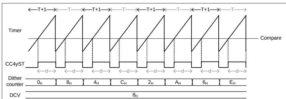
Figure 22-49 Dither timing diagram in edge aligned - \text{CC4yTC.DITHE} = 11_B
