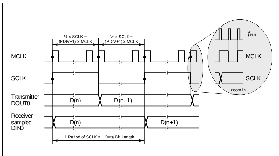
Figure 17-63 MCLK and SCLK for IIS
