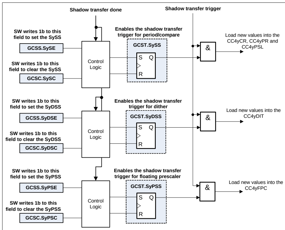
Figure 22-9 Shadow transfer enable logic
