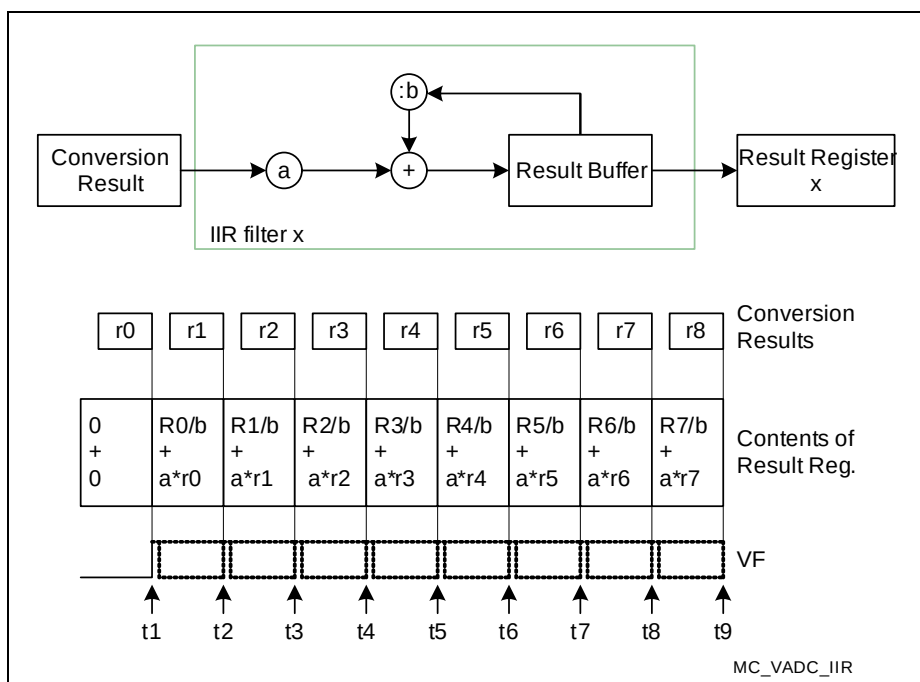
Figure 19-21 IIR Filter Structure
