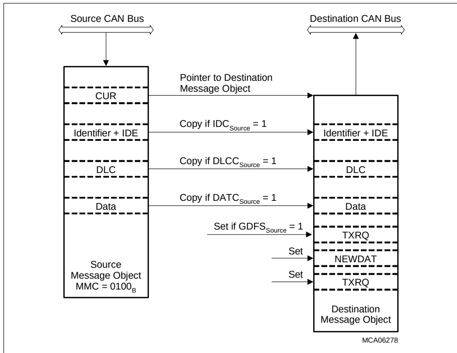
Figure 18-20 Gateway Transfer from Source to Destination
