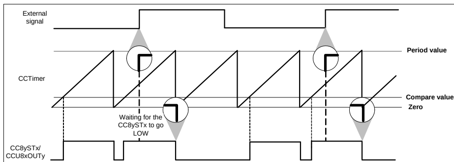
Figure 23-45 External modulation clearing the ST bit - \text{CC8yTC.EMS} = 1_B
