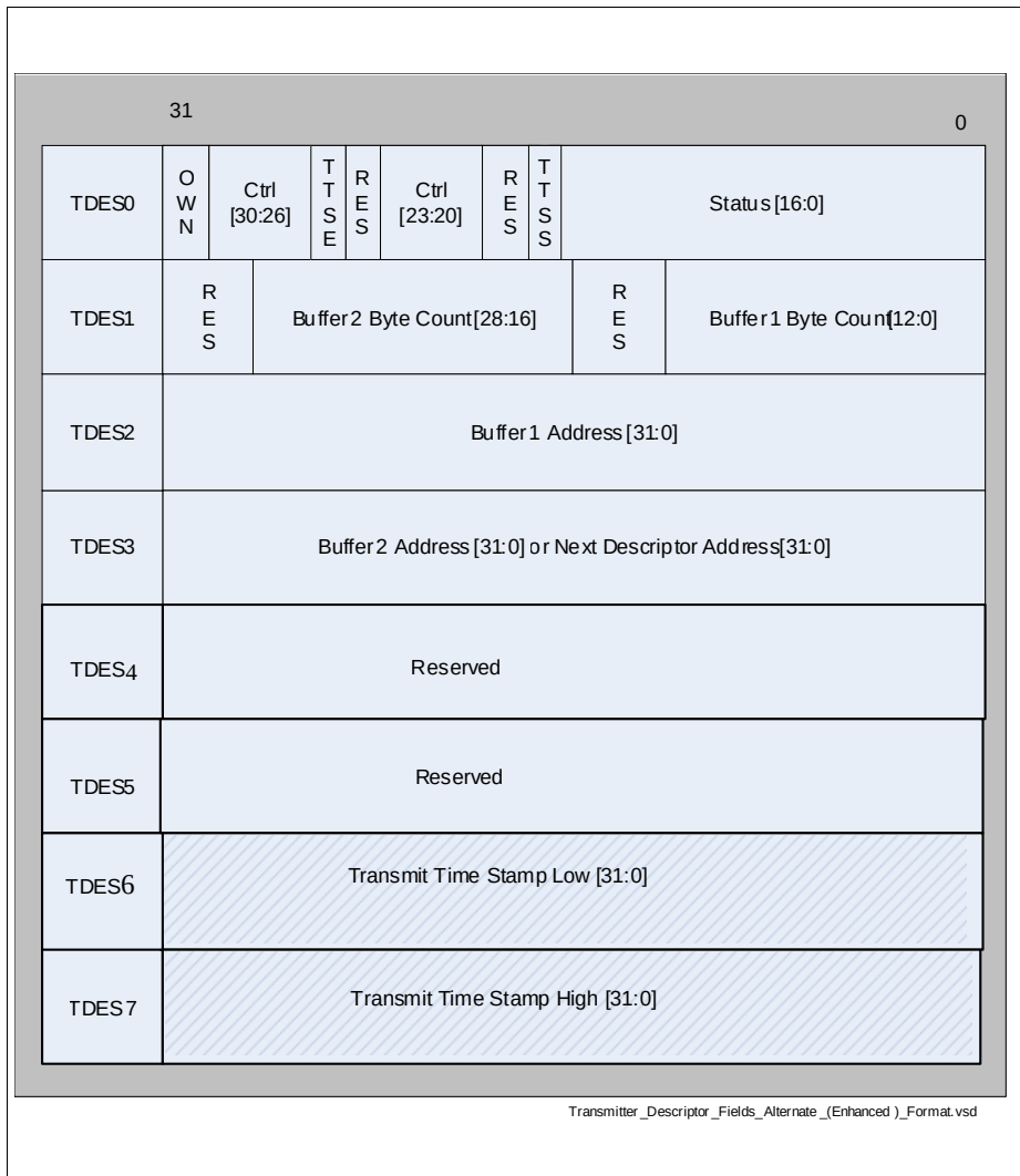
Figure 15-11 Transmitter Descriptor Fields - Alternate (Enhanced) Format
