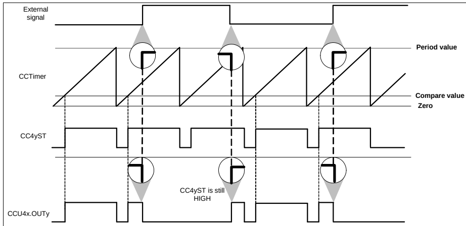
Figure 22-31 External modulation gating the output - \text{CC4yTC.EMT} = 1_B
