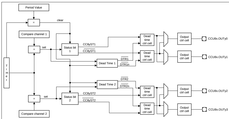
Figure 23-21 Edge Aligned with two independent channels scheme
