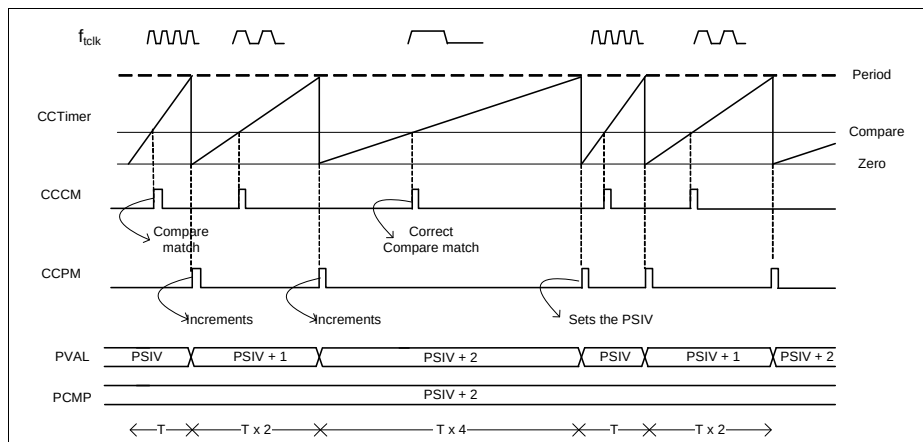
Figure 22-60 Floating Prescaler compare mode usage - Edge Aligned
