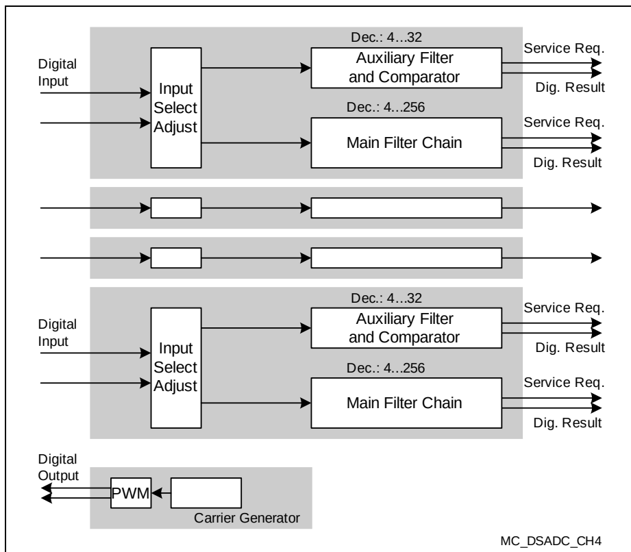
Figure 20-1 DSD Module Overview
