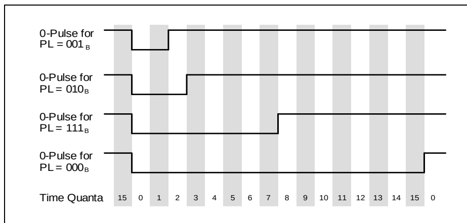
Figure 17-33 Transmitter Pulse Length Control
