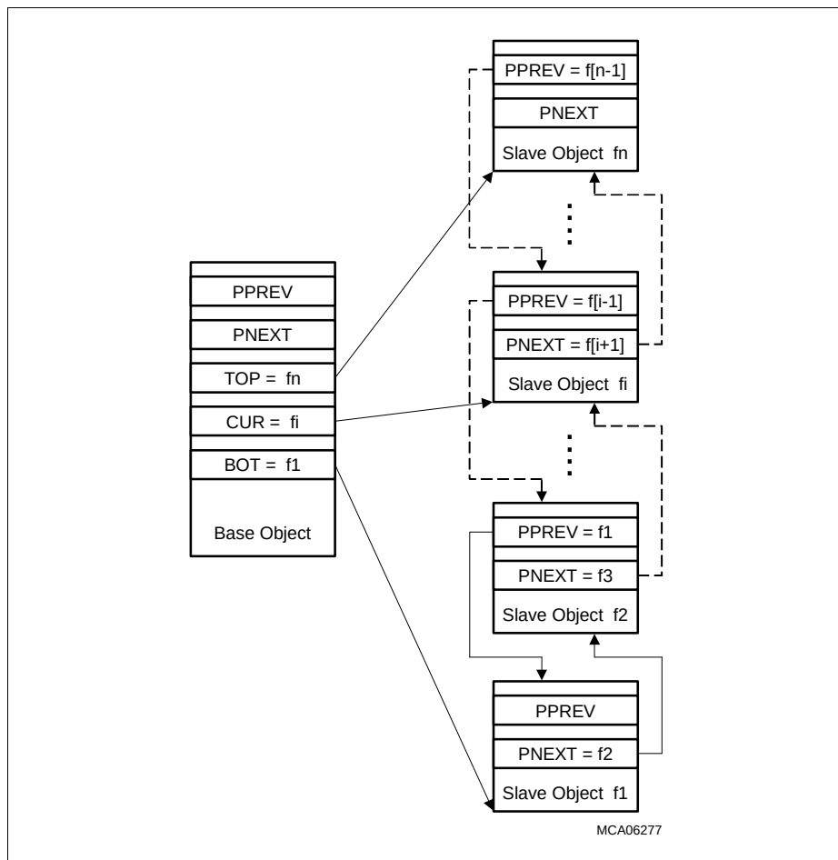
Figure 18-19 FIFO Structure with FIFO Base Object and n FIFO Slave Objects
