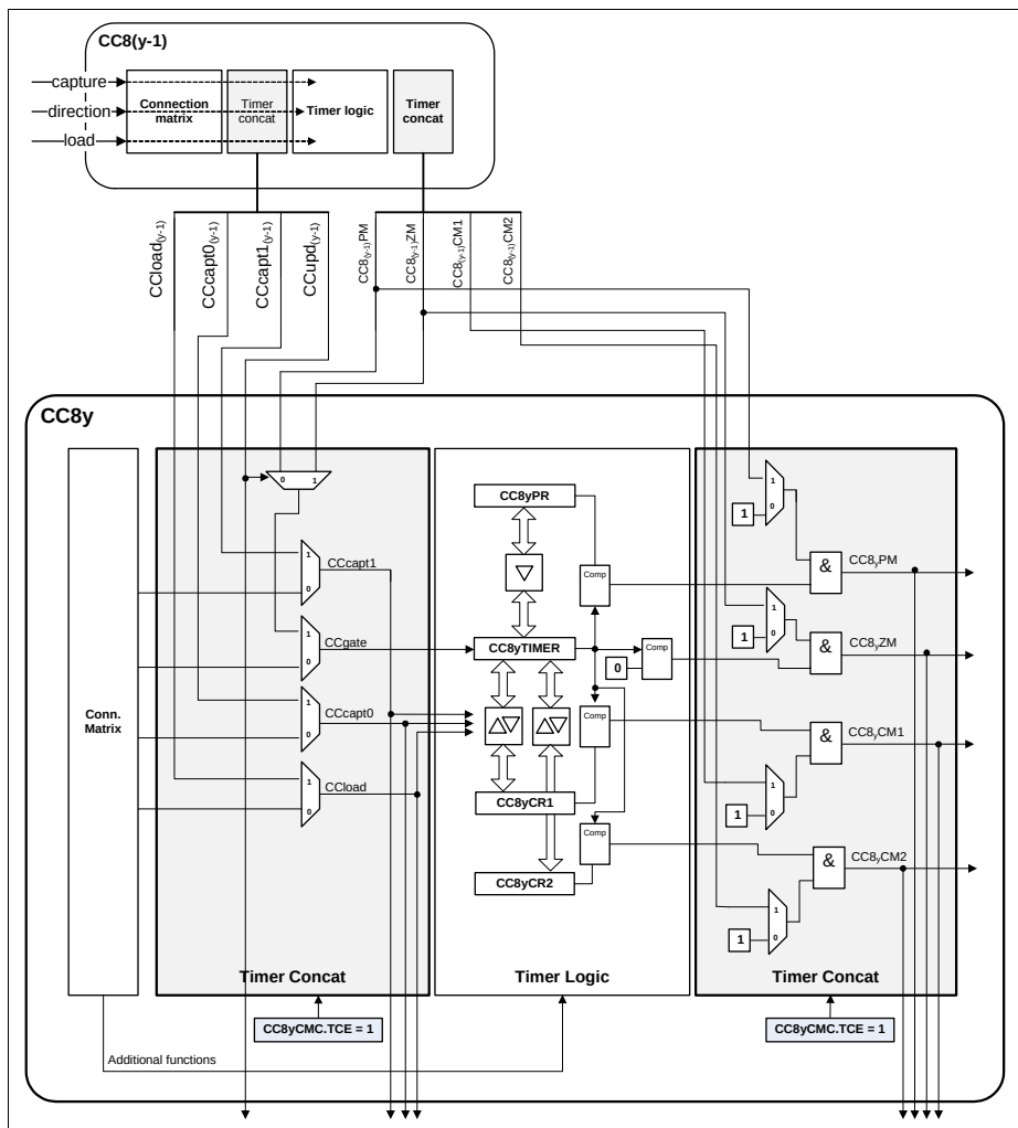
Figure 23-60 Timer concatenation control logic
