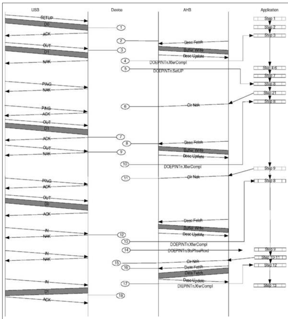
Figure 16-40 Three-Stage Control Write
