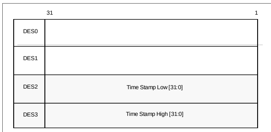
Figure 15-9 Receive Descriptor Fields When DMA Clears the Own Bit
