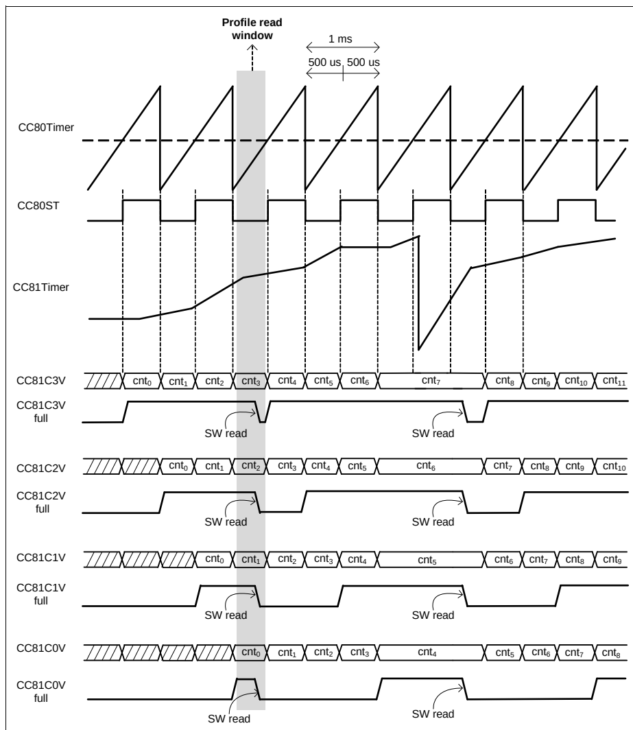
Figure 23-81 Three Capture profiles - \text{CC8yTC.SCE} = 1_b
