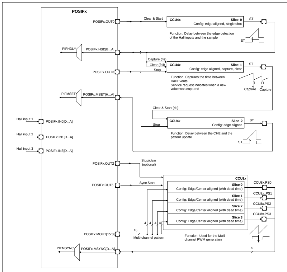
Figure 24-16 Hall Sensor Mode usage - profile 2
