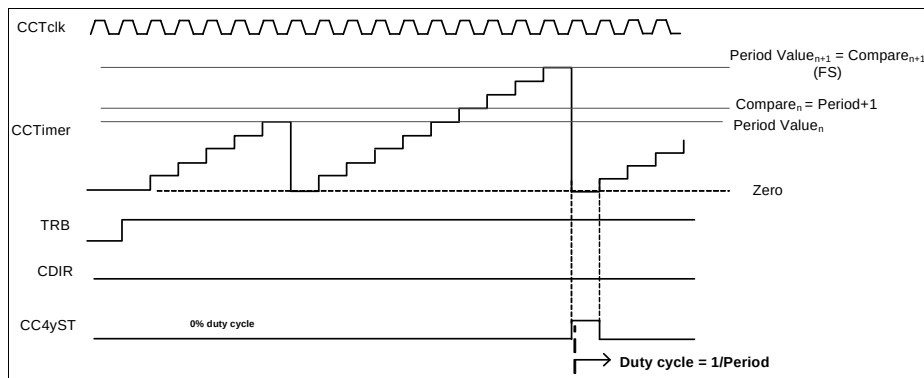
Figure 22-57 PWM with 0% duty cycle - Edge Aligned Mode
