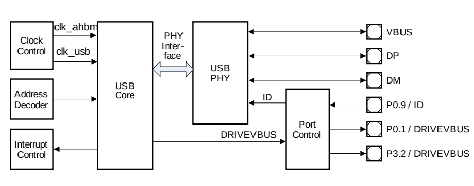
Figure 16-1 USB Module Block Diagram
