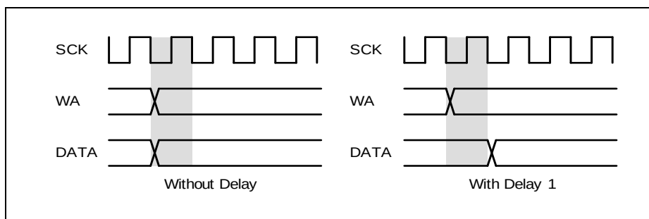
Figure 17-59 Transfer Delay for IIS
