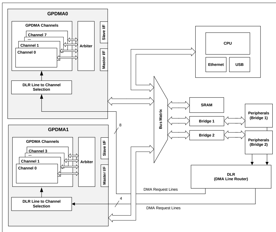
Figure 5-1 GPDMA Block Diagram
