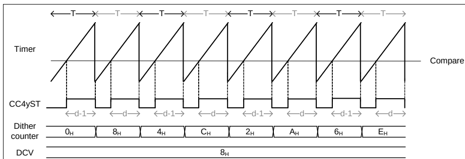
Figure 22-48 Dither timing diagram in edge aligned - \text{CC4yTC.DITHE} = 10_B
