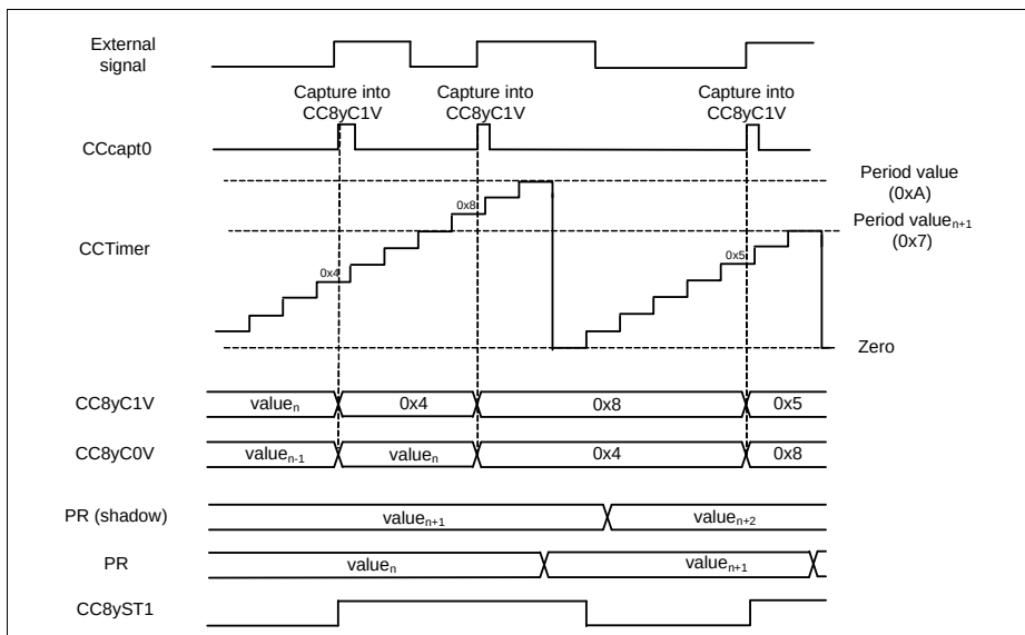
Figure 23-39 External capture - \text{CC8yCMC.CAP0S} \neq 00_{\text{B}} , \text{CC8yCMC.CAP1S} = 00_{\text{B}}
