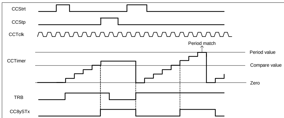
Figure 23-32 Start (as flush and start)/ stop (as stop) - CC8yTC.STRM = 1_B , CC8yTC.ENDM = 00_B
