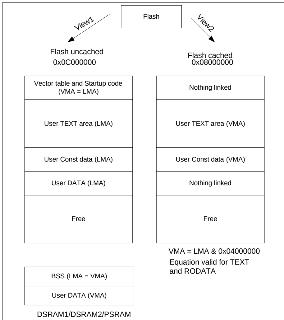
Figure 26-5 Memory Layout2
