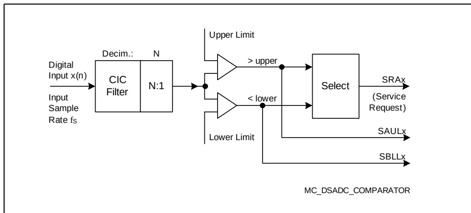
Figure 20-10 Comparator Structure
