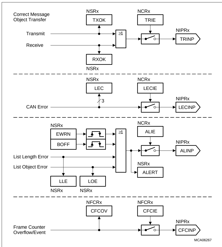
Figure 18-9 CAN Node Interrupts
