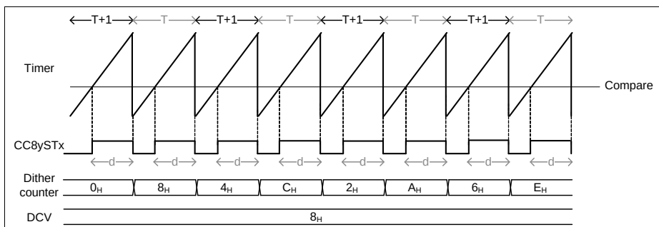
Figure 23-67 Dither timing diagram in edge aligned - \text{CC8yTC.DITHE} = 11_B
