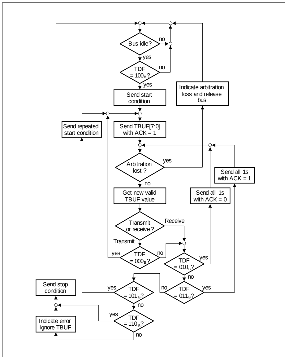
Figure 17-55 IIC Master Transmission
