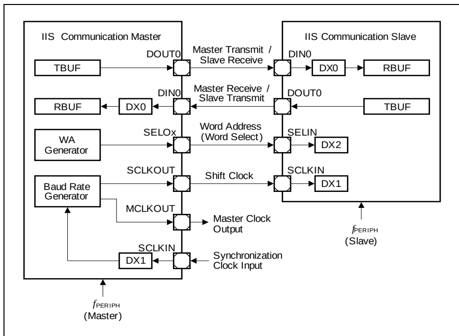
Figure 17-57 IIS Signals
