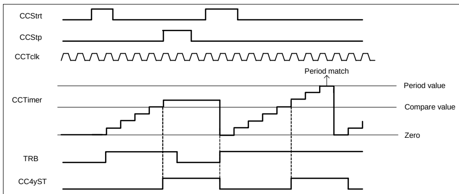
Figure 22-18 Start (as flush and start)/ stop (as stop) - \text{CC4yTC.STRM} = 1_{\text{B}} , \text{CC4yTC.ENDM} = 00_{\text{B}}
