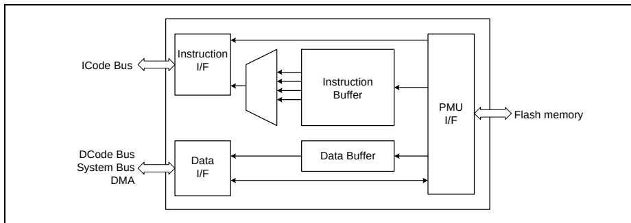
Figure 8-2 Prefetch Unit
