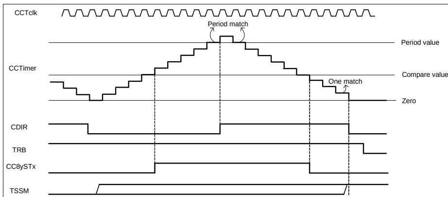
Figure 23-15 Single shot center aligned - CC8yTC.TSSM = 1 B , CC8yTC.TCM = 1 B
