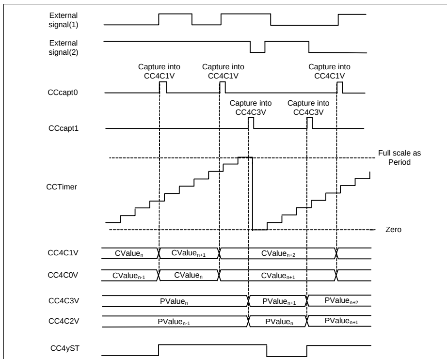
Figure 22-25 External capture - CC4yCMC.CAP0S \neq 00_B , CC4yCMC.CAP1S \neq 00_B
