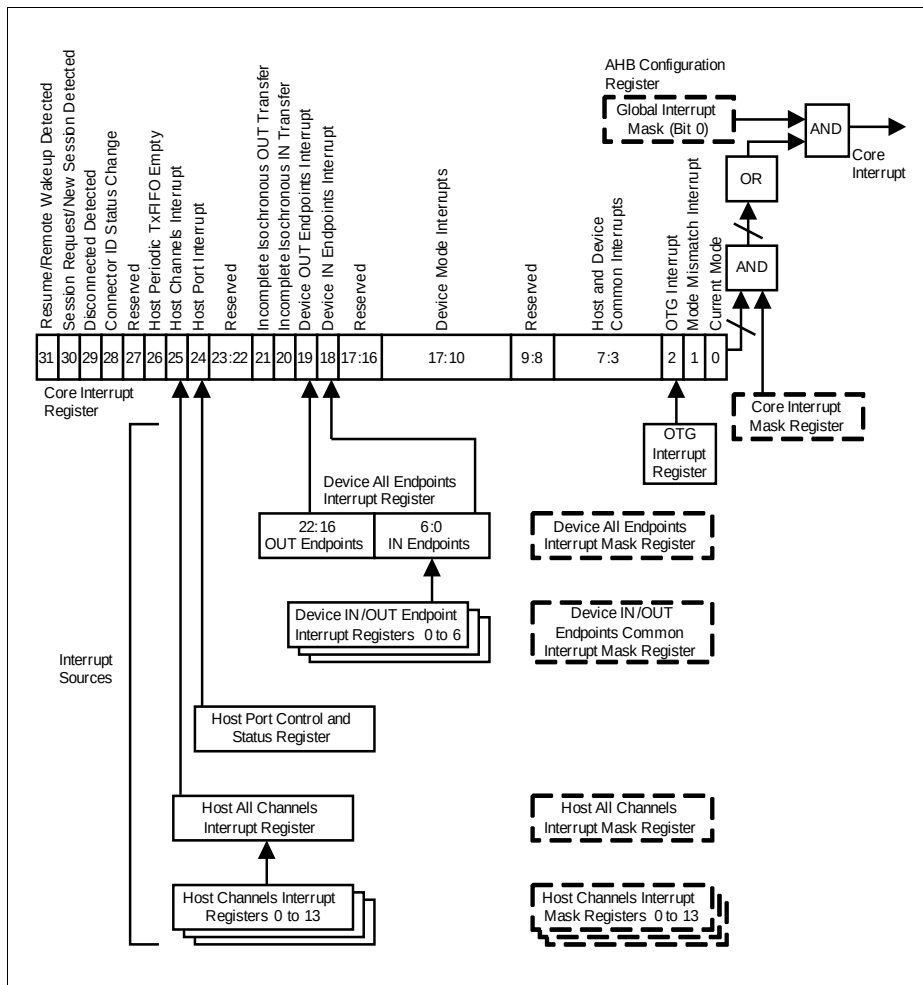
Figure 16-71 Interrupt Hierarchy
