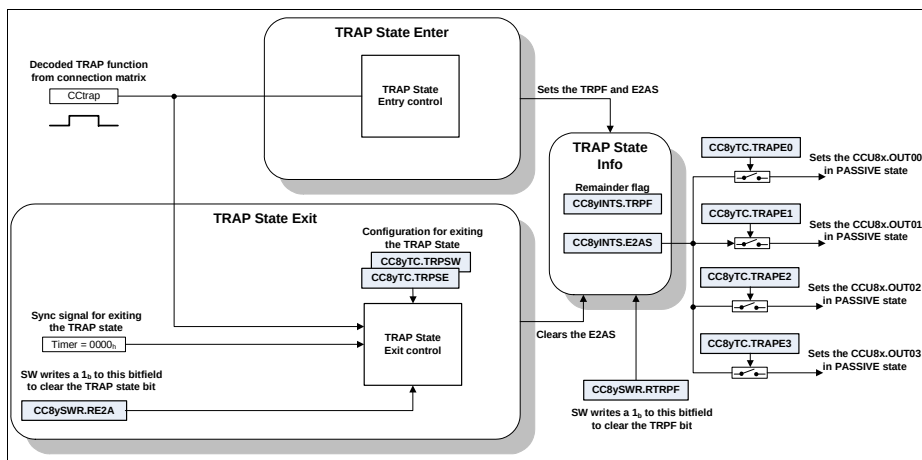
Figure 23-47 Trap control diagram
