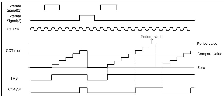
Figure 22-19 Start (as start)/ stop (as flush and stop) - \text{CC4yTC.STRM} = 0_{\text{B}} , \text{CC4yTC.ENDM} = 10_{\text{B}}
