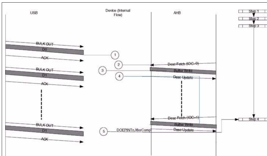
Figure 16-57 Bulk OUT Transfers
