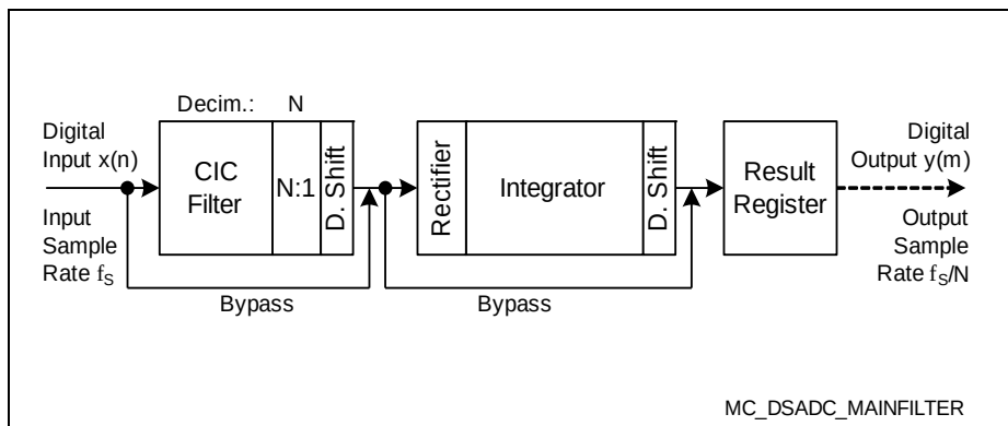
Figure 20-7 Structure of the Main Filter Chain
