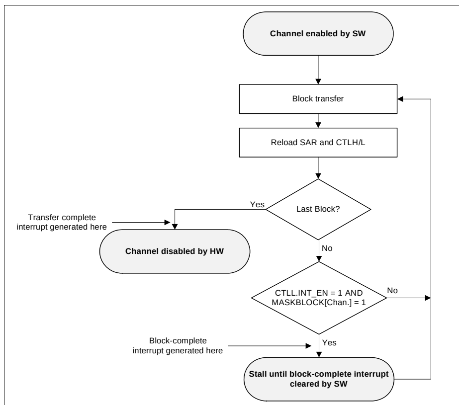
Figure 5-19 DMA Transfer Flow for Source Address Auto-Reloaded and Linked List Destination Address
