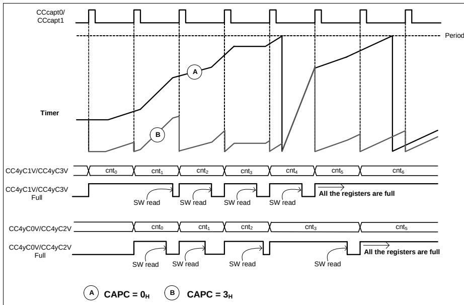
Figure 22-62 Capture mode usage - single channel
