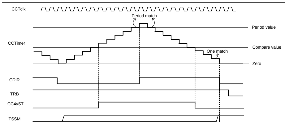
Figure 22-15 Single shot center aligned - CC4yTC.TSSM = 1_B , CC4yTC.TCM = 1_B
