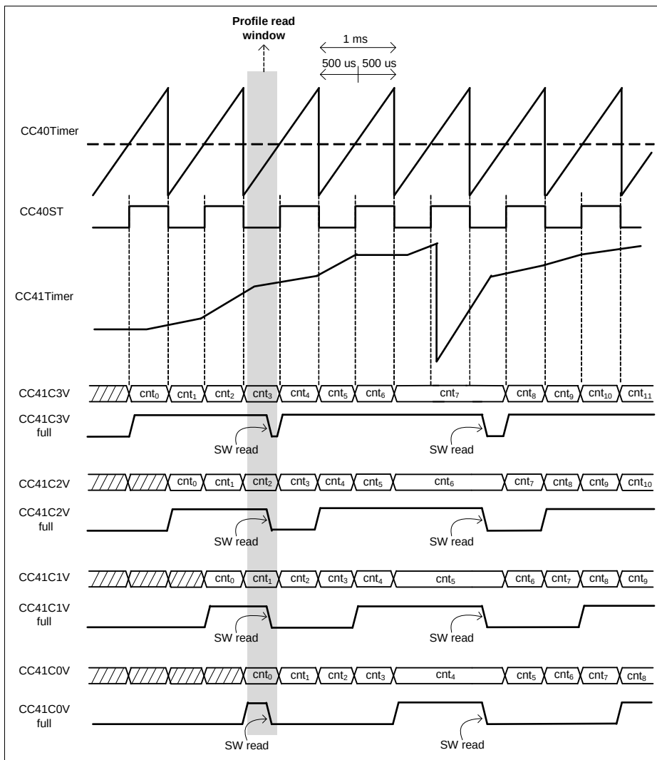
Figure 22-63 Three Capture profiles - CC4yTC.SCE = 1 B
