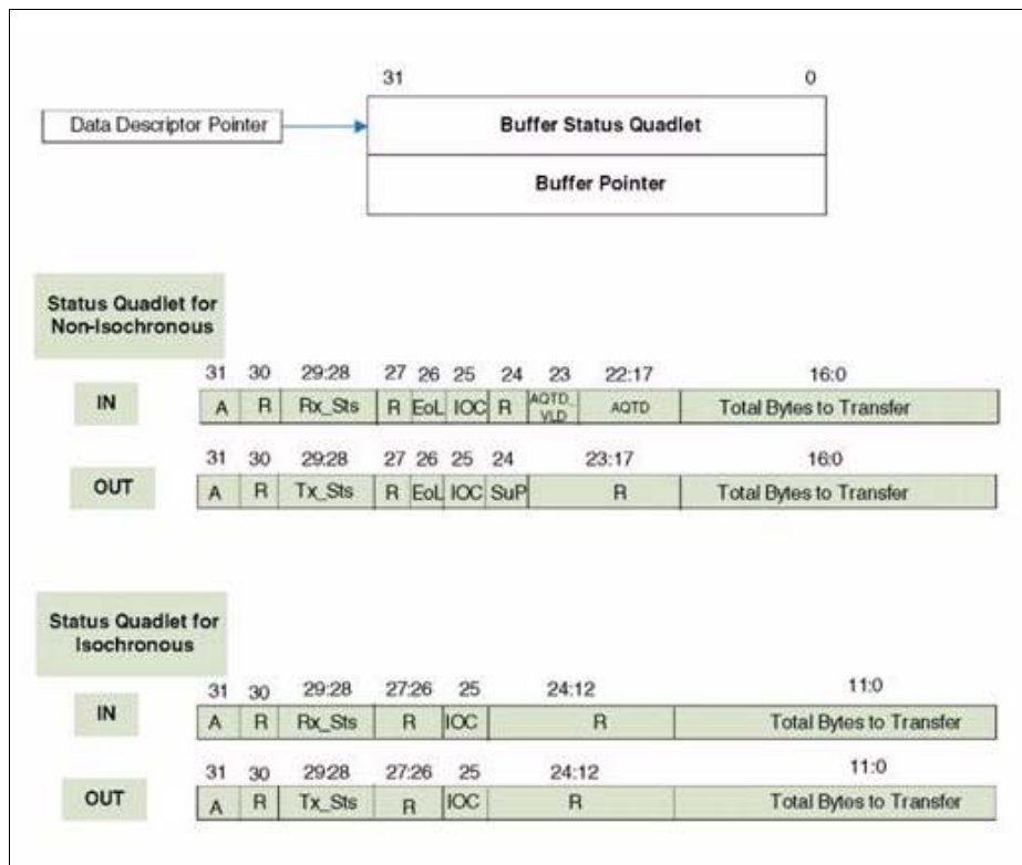
Figure 16-19 Memory Structure
