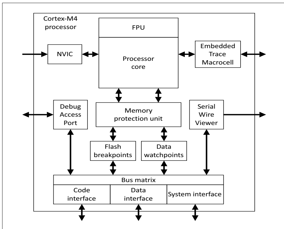
Figure 2-1 Cortex-M4 Block Diagram
