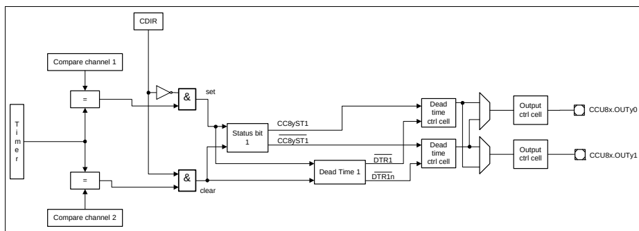
Figure 23-28 Center Aligned Asymmetric mode scheme
