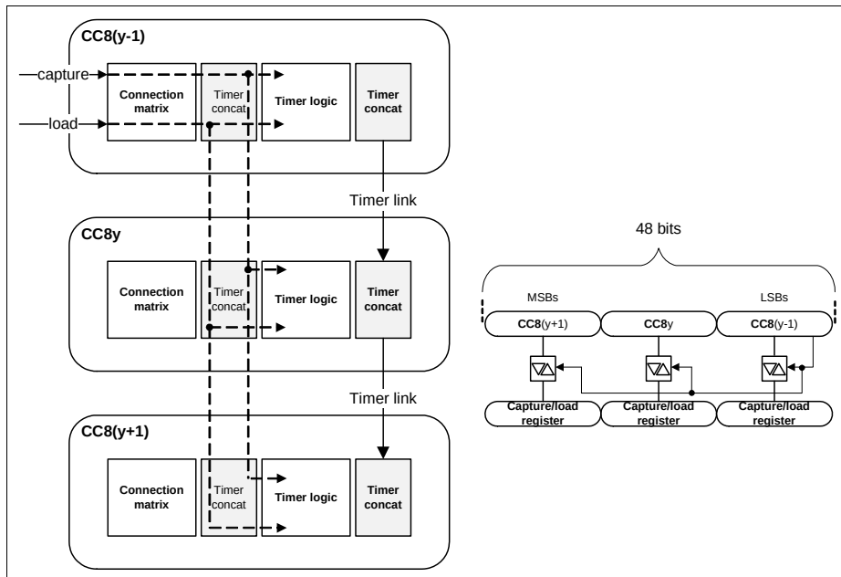
Figure 23-58 Capture/Load Timer Concatenation
