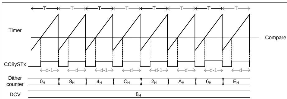
Figure 23-66 Dither timing diagram in edge aligned - \text{CC8yTC.DITHE} = 10_B
