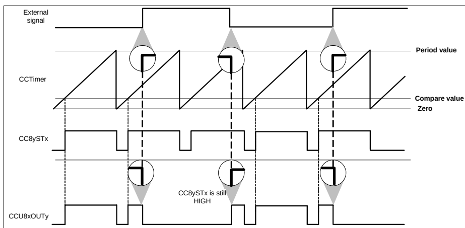
Figure 23-46 External modulation gating the output - \text{CC8yTC.EMT} = 1_B
