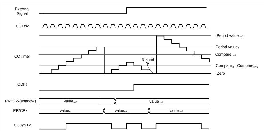
Figure 23-34 External counting direction
