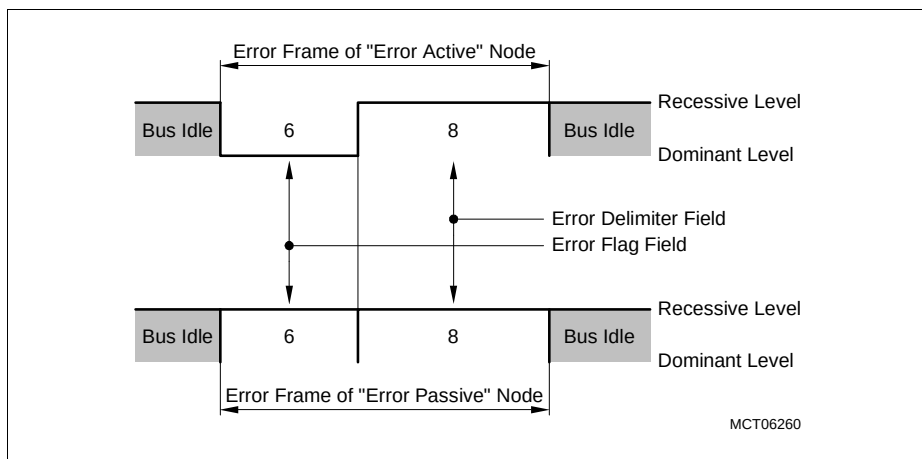
Figure 18-4 CAN Error Frames
