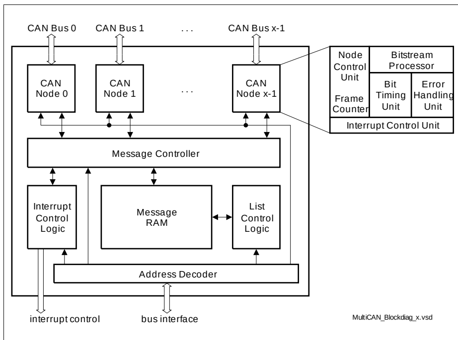
Figure 18-6 MultiCAN Block Diagram
