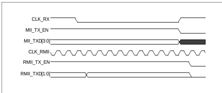
Figure 15-24 End of MII and RMII Transmission in 10 Mbit/s Mode
