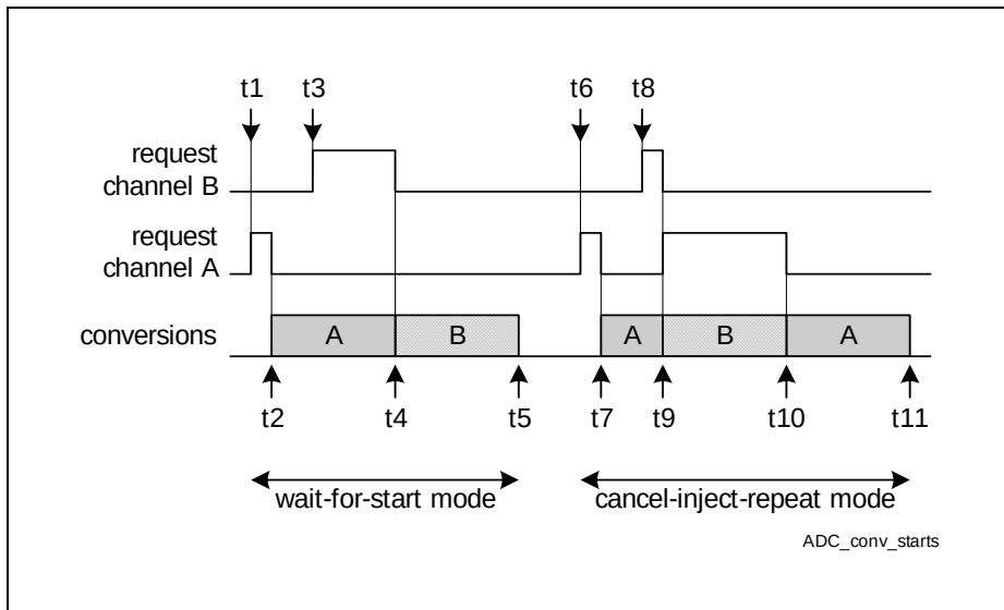
Figure 19-9 Conversion Start Modes
