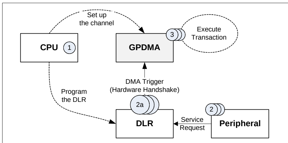
Figure 5-4 Hardware Handshaking Interface
