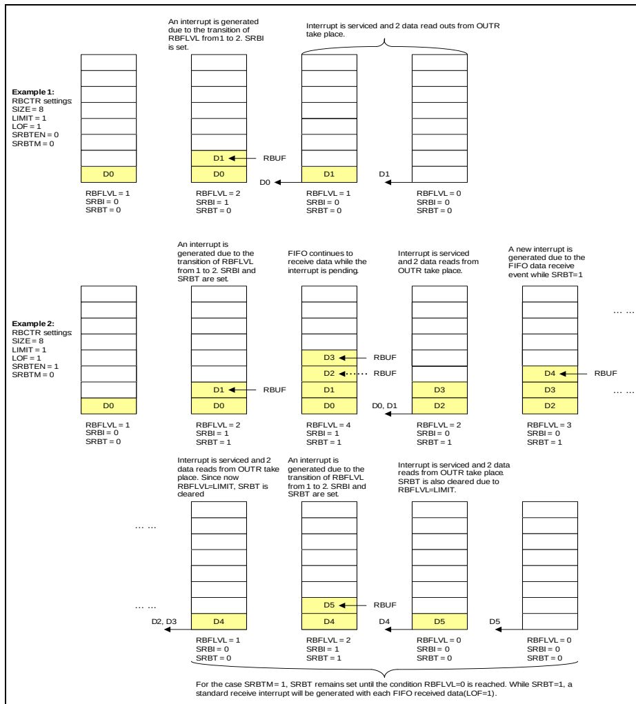
Figure 17-24 Standard Receive Buffer Event Examples
