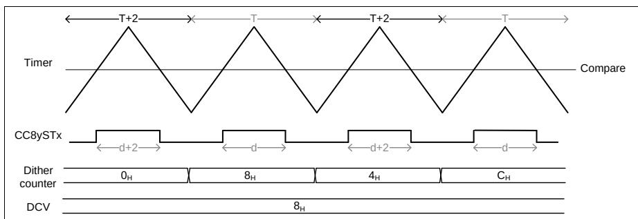
Figure 23-68 Dither timing diagram in center aligned - \text{CC8yTC.DITHE} = 01_B
