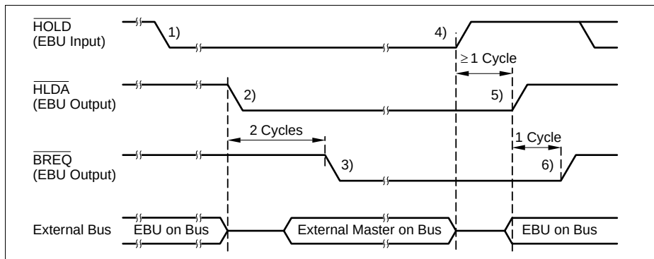
Figure 14-12 Arbitration Sequence with the EBU in Arbiter Mode
