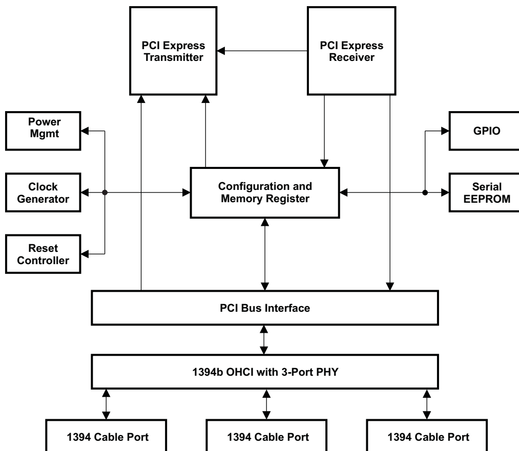
Figure 3-1. XIO2213B Block Diagram
