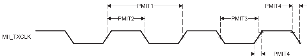
Figure 5-68. PRU-ICSS MII_TXCLK Timing
