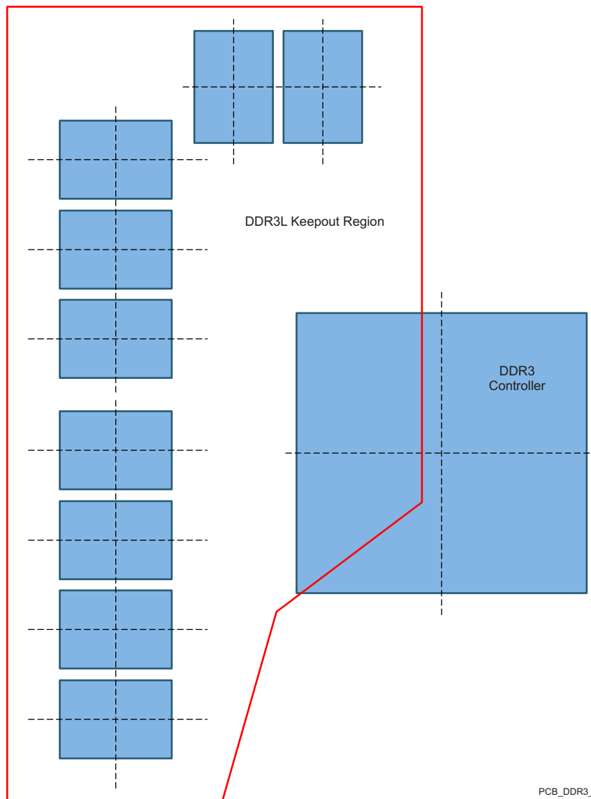
Figure 7-5. DDR3L Keepout Region
