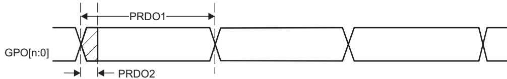
Figure 5-56. PRU-ICSS PRU Direct Output Timing
