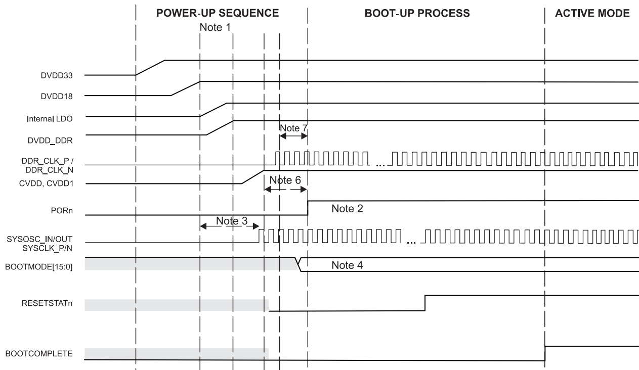
Figure 5-1. Power-Up Sequencing
