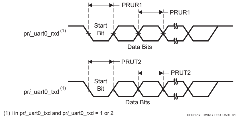
Figure 5-71. PRU-ICSS UART Timing
