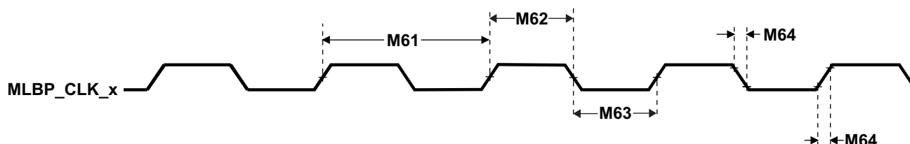
Figure 5-48. MLB_CLKP/N Timing (1)
