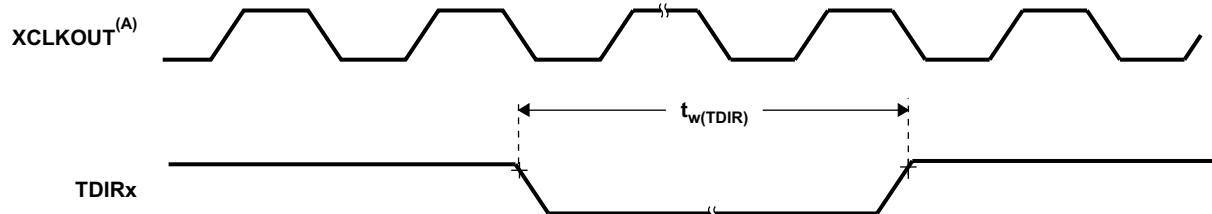
Figure 6-19. TDIRx Timing
