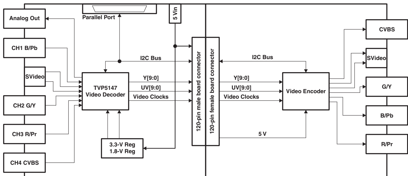
Figure 1-3. TVP5147EVM
