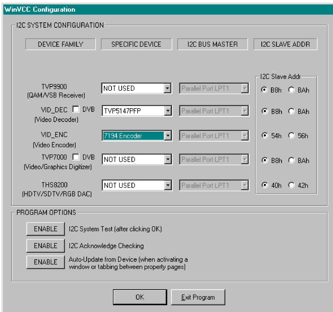
Figure 3-1. WinVCC I 2 C Address Configuration
