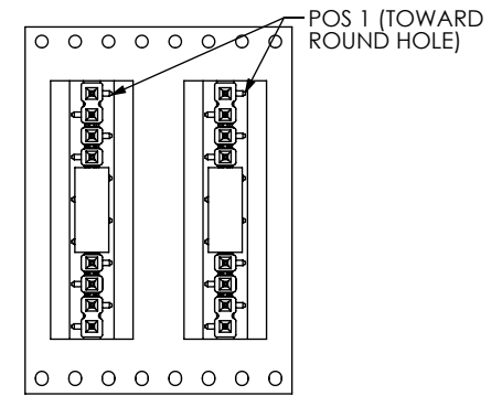
FIG 5 -TR: TAPE & REEL PACKAGING OPTION
