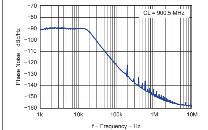
Figure 31. Closed Loop VCO Phase Noise
