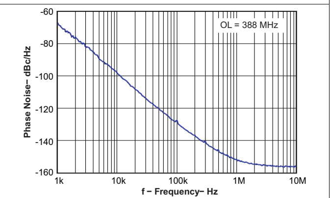
Figure 7. Open Loop VCO Phase Noise
