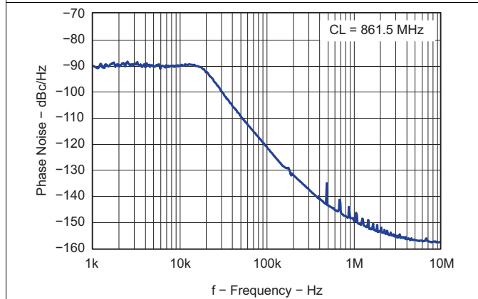
Figure 22. Closed Loop VCO Phase Noise
