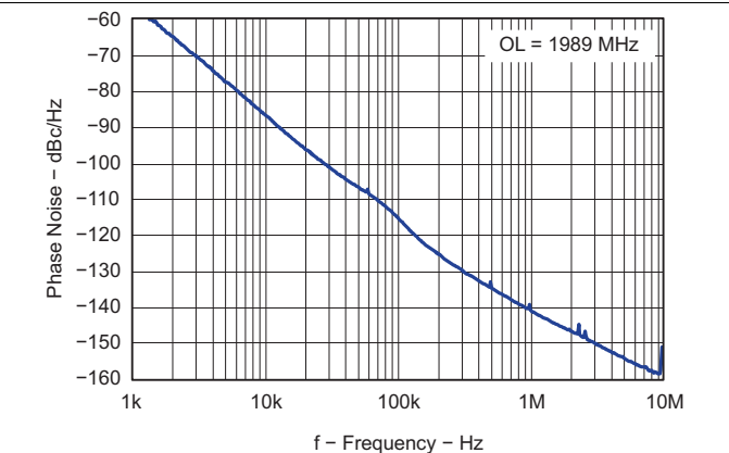
Figure 57. Open Loop VCO Phase Noise
