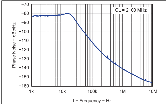
Figure 65. Closed Loop VCO Phase Noise
