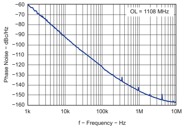
Figure 77. Open Loop VCO Phase Noise
