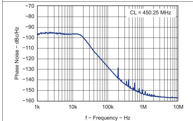
Figure 33. Closed Loop VCO Phase Noise
