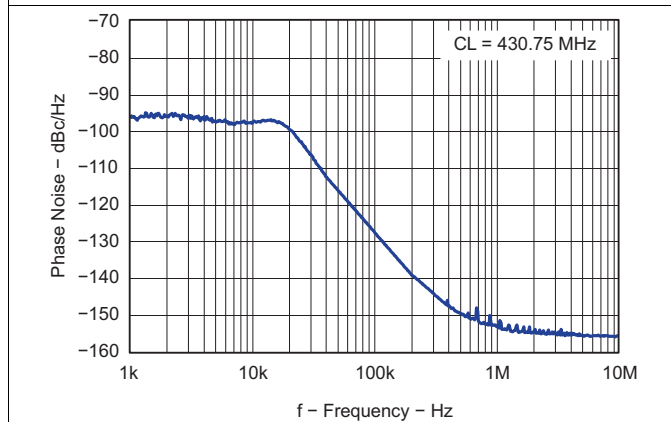
Figure 24. Closed Loop VCO Phase Noise
