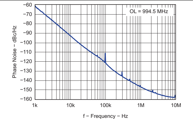
Figure 59. Open Loop VCO Phase Noise
