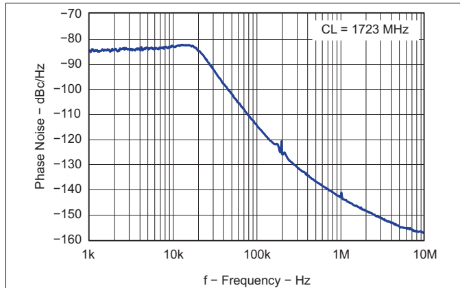
Figure 20. Closed Loop VCO Phase Noise
