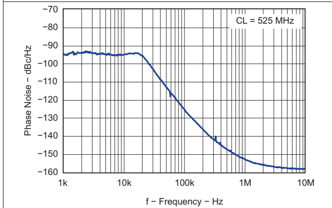
Figure 69. Closed Loop VCO Phase Noise
