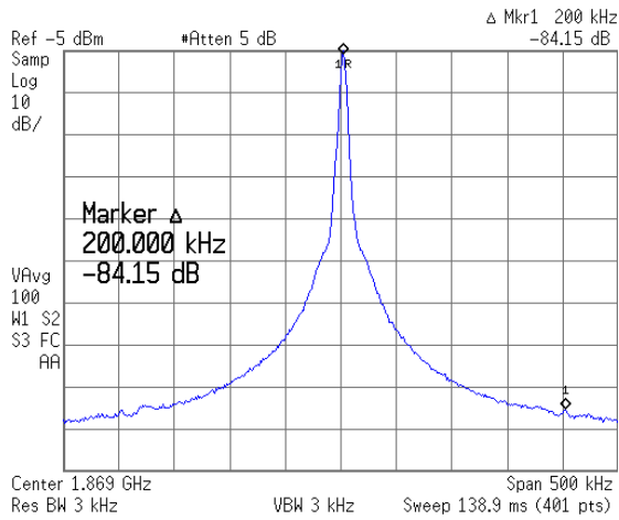
Figure 44. Direct Output: PFD Frequency Spurs
