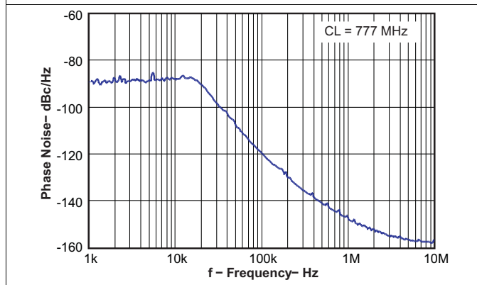
Figure 4. Closed Loop VCO Phase Noise
