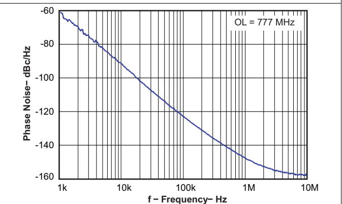
Figure 5. Open Loop VCO Phase Noise
