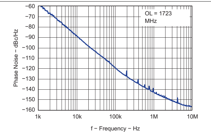
Figure 21. Open Loop VCO Phase Noise
