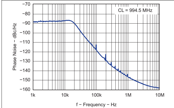
Figure 58. Closed Loop VCO Phase Noise
