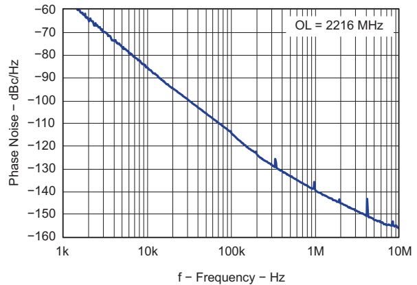
Figure 75. Open Loop VCO Phase Noise
