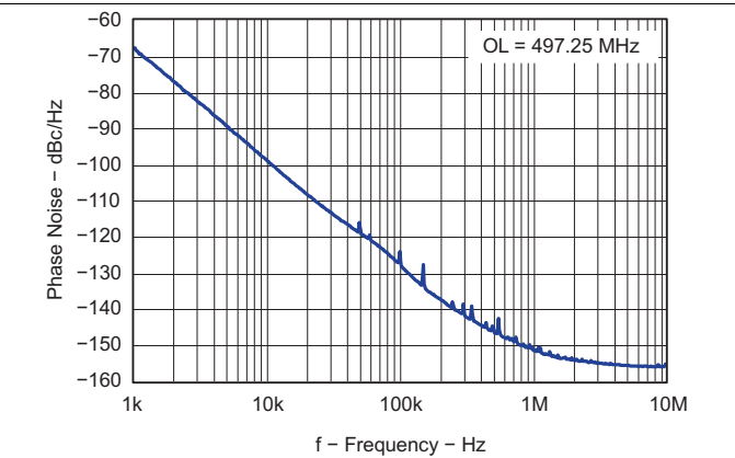
Figure 61. Open Loop VCO Phase Noise
