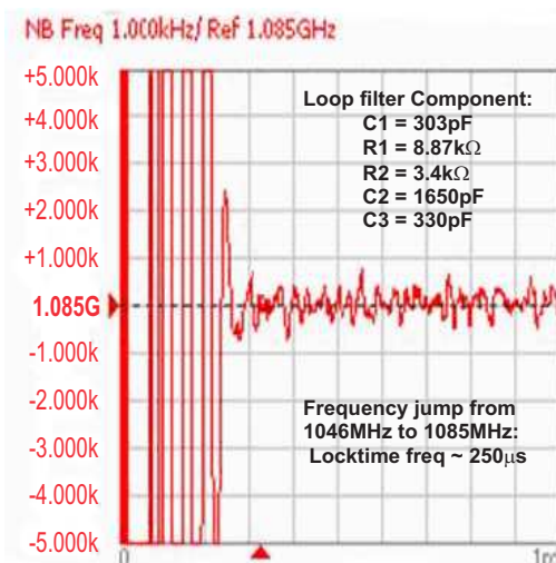
Figure 88. Frequency Locktime
