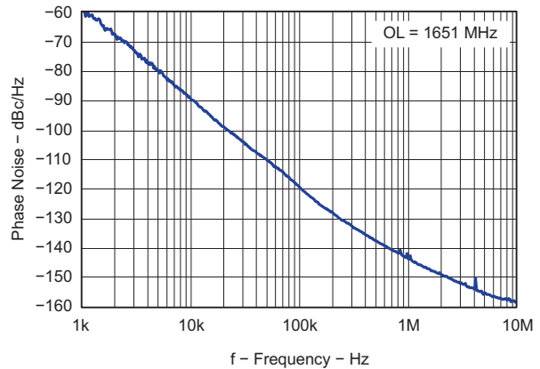
Figure 12. Open Loop VCO Phase Noise
