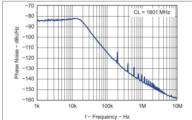
Figure 29. Closed Loop VCO Phase Noise
