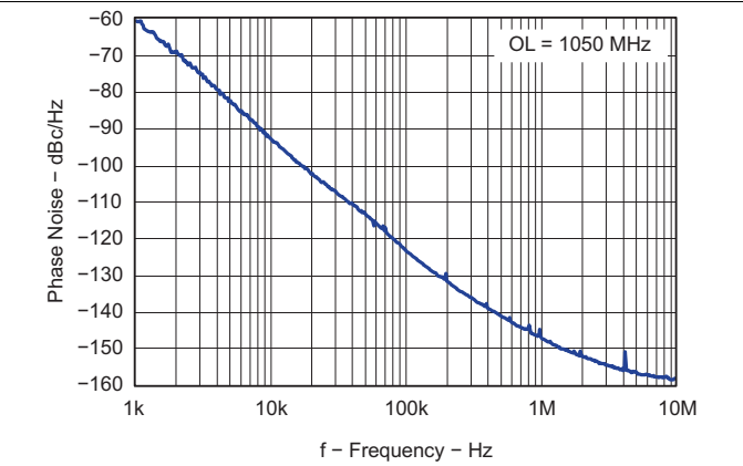
Figure 68. Open Loop VCO Phase Noise
