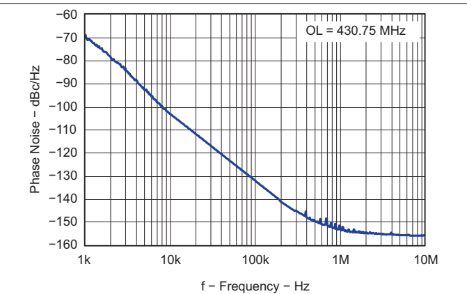
Figure 25. Open Loop VCO Phase Noise
