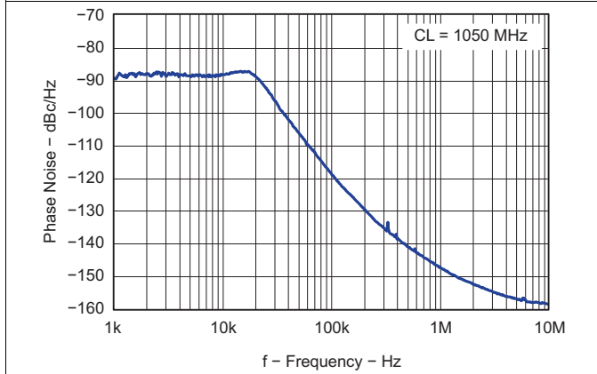
Figure 67. Closed Loop VCO Phase Noise
