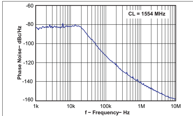
Figure 2. Closed Loop VCO Phase Noise
