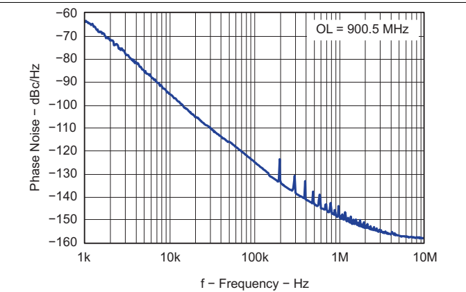
Figure 32. Open Loop VCO Phase Noise
