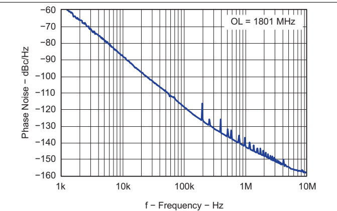
Figure 30. Open Loop VCO Phase Noise
