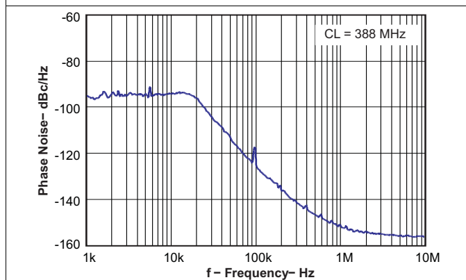
Figure 6. Closed Loop VCO Phase Noise
