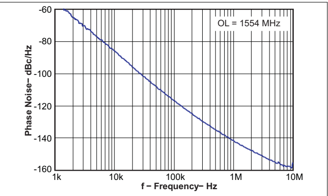
Figure 3. Open Loop VCO Phase Noise
