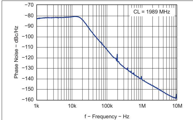
Figure 56. Closed Loop VCO Phase Noise
