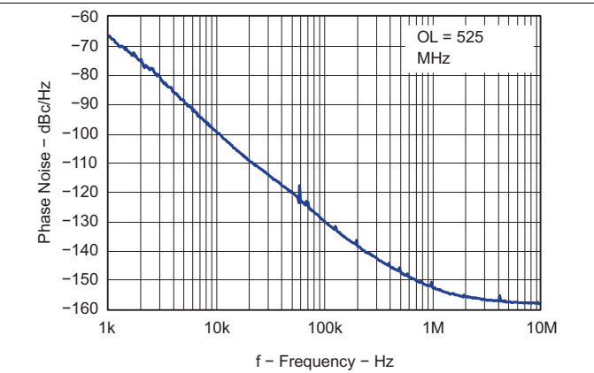
Figure 70. Open Loop VCO Phase Noise
