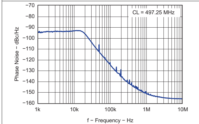
Figure 60. Closed Loop VCO Phase Noise
