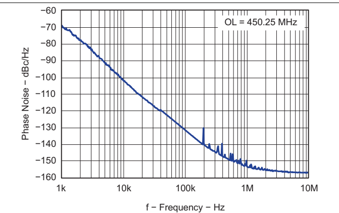
Figure 34. Open Loop VCO Phase Noise
