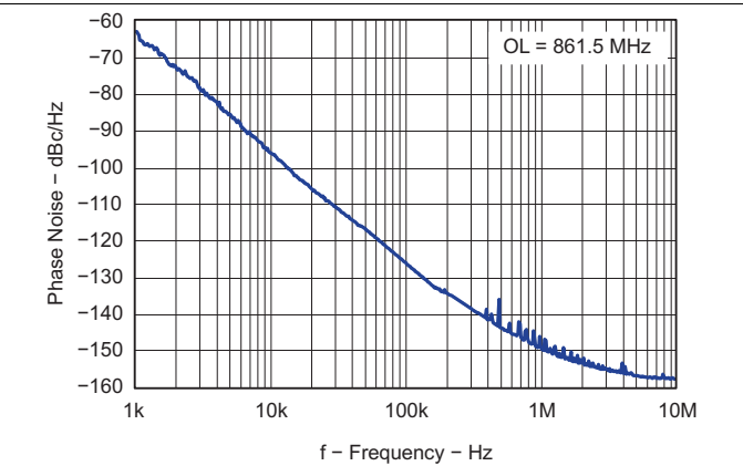
Figure 23. Open Loop VCO Phase Noise
