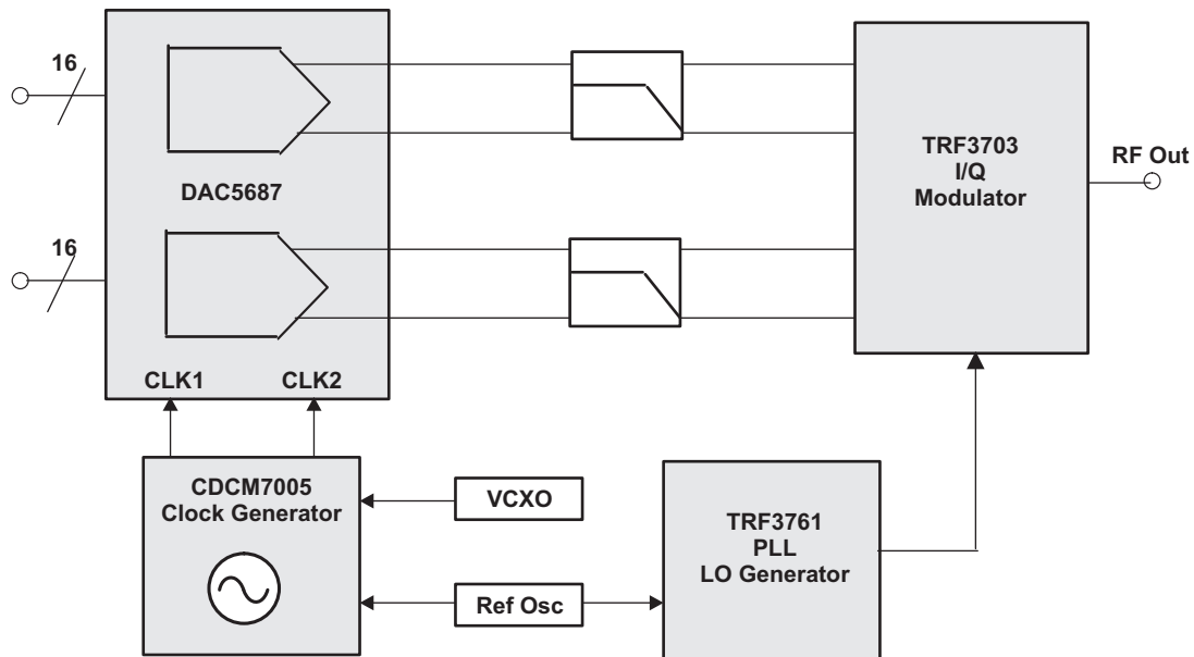
Figure 90. Transmit Chain Block Diagram
