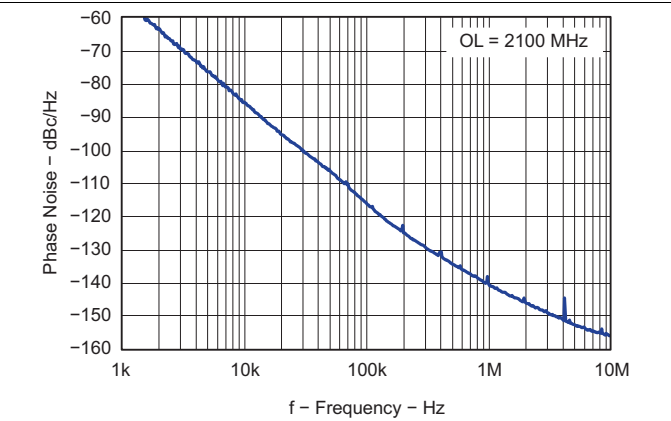
Figure 66. Open Loop VCO Phase Noise
