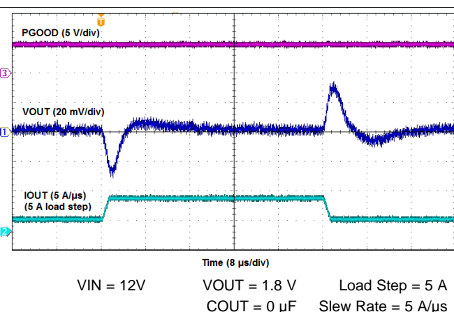
Figure 15. Transient Response
