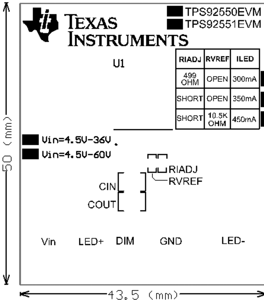
Figure 41. Top Overlay
