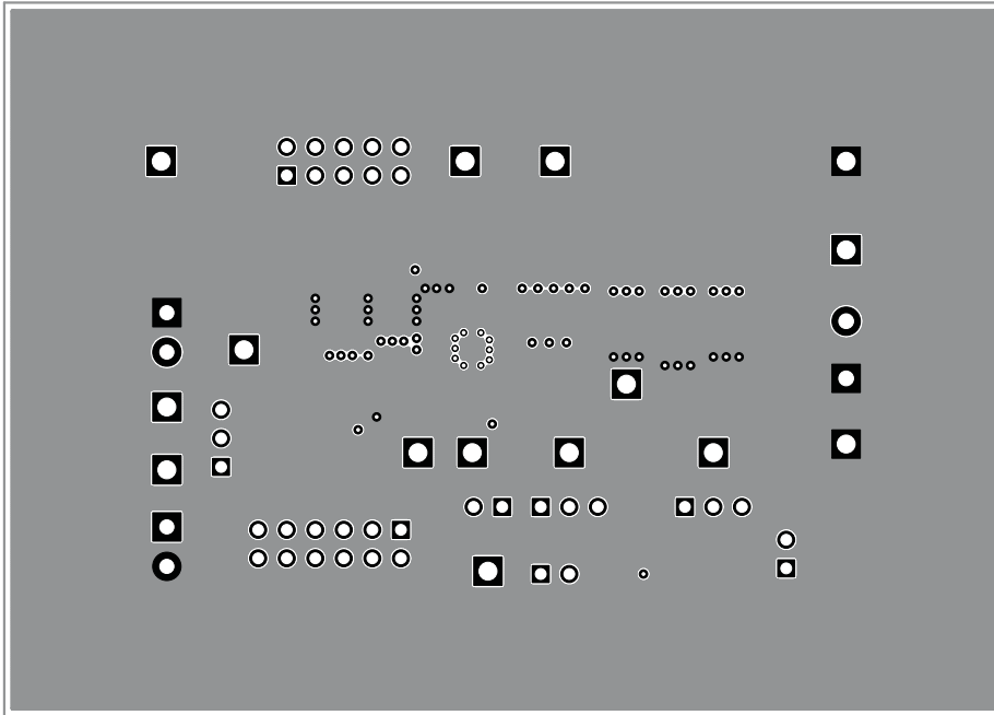
Figure 15. TPS84x2xEVM-692 Layer 3
