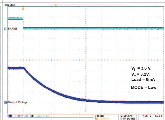
Figure 26. TPS82699 Shutdown
