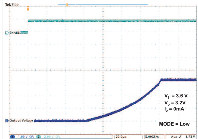
Figure 24. TPS82699 Start-Up
