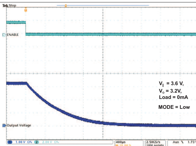
Figure 26. TPS82699 Shutdown
