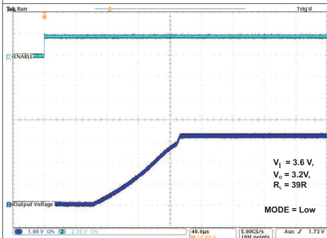
Figure 25. TPS82699 Start-Up
