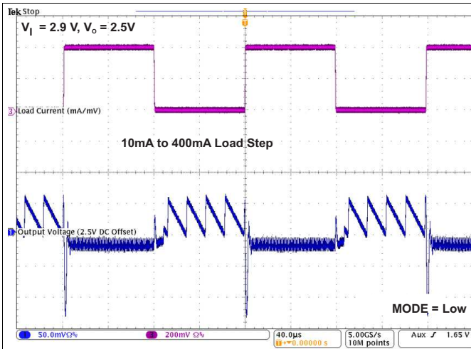
Figure 32. TPS826951 Load Transient Response In PFM/PWM Operation
