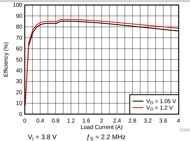
Figure 4-5. SMPS Efficiency for 4-A Multi-Phase PWM Mode
