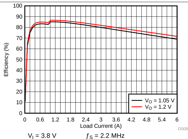
Figure 4-6. SMPS Efficiency for 6-A Multi-Phase PWM Mode
