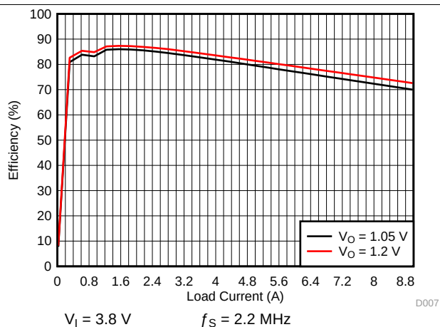
Figure 4-7. SMPS Efficiency for 9-A Multi-Phase PWM Mode
