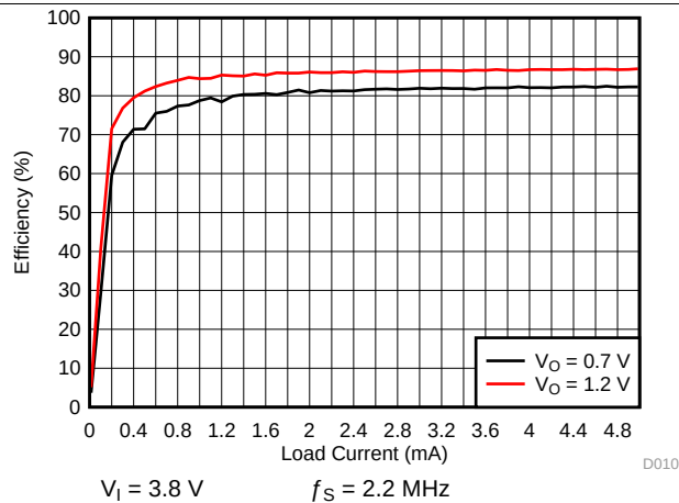
Figure 4-4. SMPS Efficiency for Multi-Phase Eco-mode
