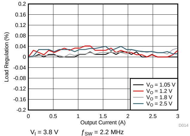
Figure 6-10. SMPS Load Regulation for 3-A Single Phase
