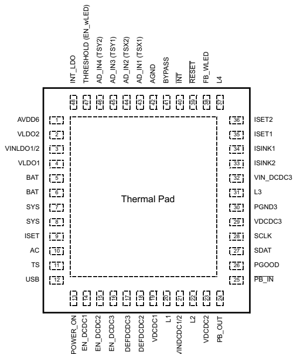
TPS6507x RSL Package 48-Pin VQFN With Thermal Pad Top View
