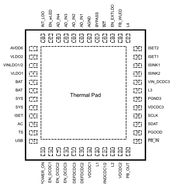
TPS65072 RSL Package 48-Pin VQFN With Thermal Pad Top View
