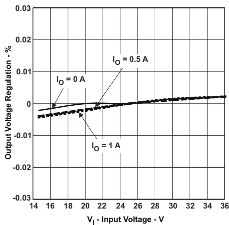
Figure 7-13. Output Voltage Regulation % vs Input Voltage
