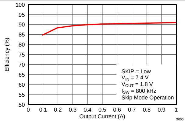
Figure 14. Efficiency vs Output Current, SKIP = Low
