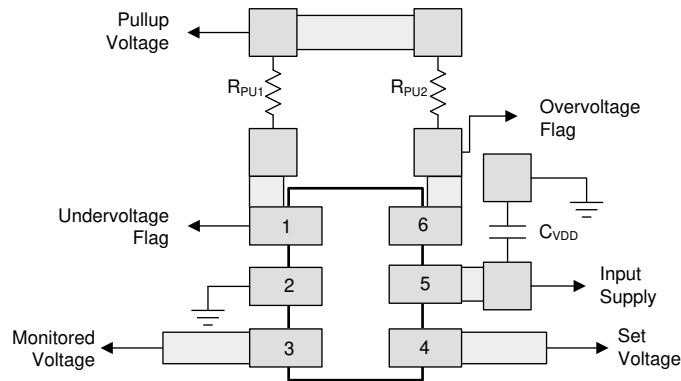
Figure 9-1. Recommended Layout
