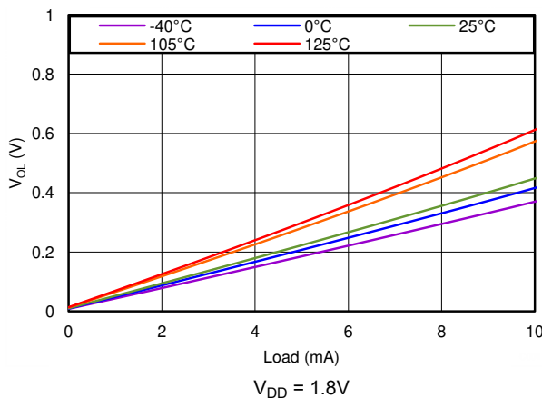
V_{DD} = 1.8\text{V} Figure 5-12. Low-Level Output Voltage vs Output Current
