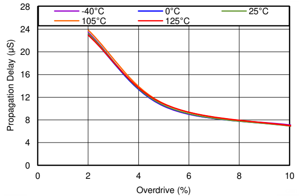
SENSE transitions from high to low Figure 5-11. Overvoltage Propagation Delay vs Overdrive
