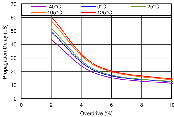
SENSE transitions from low to high Figure 5-10. Undervoltage Propagation Delay vs Overdrive
