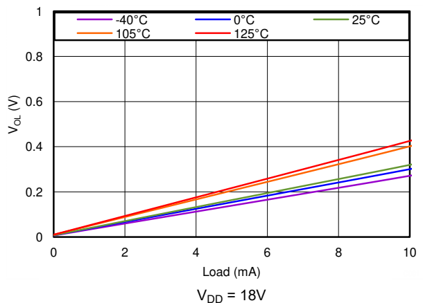
V_{DD} = 18\text{V} Figure 5-13. Low-Level Output Voltage vs Output Current
