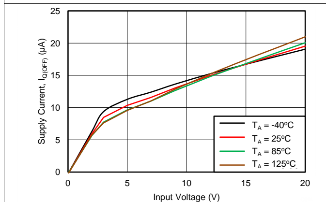
Figure 3. Input Supply Current vs Supply Voltage at Shutdown
