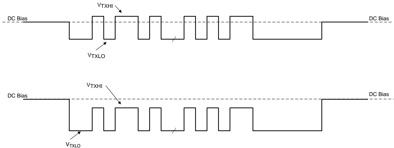
Figure 26. USB Power Delivery BMC Transmission on the CC Line
