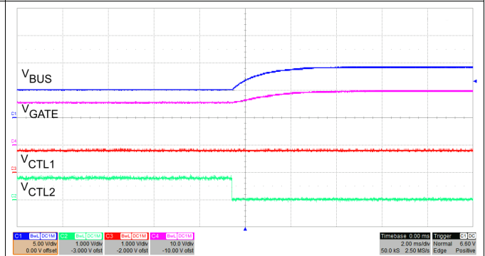
Figure 59. VBUS 5 V – 12 V Transition, TPS25741
