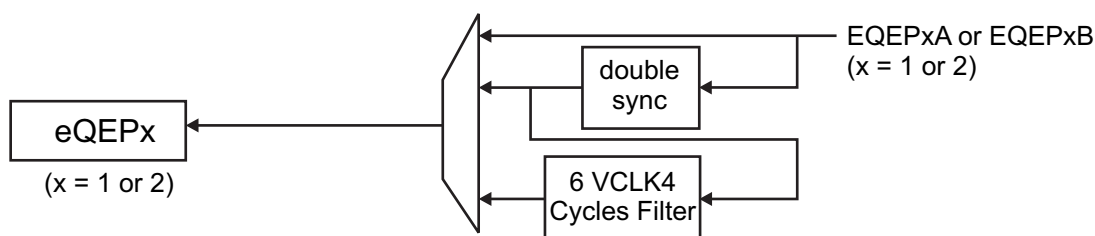
Figure 7-9. eQEPx Input Synchronization Selection Detail
