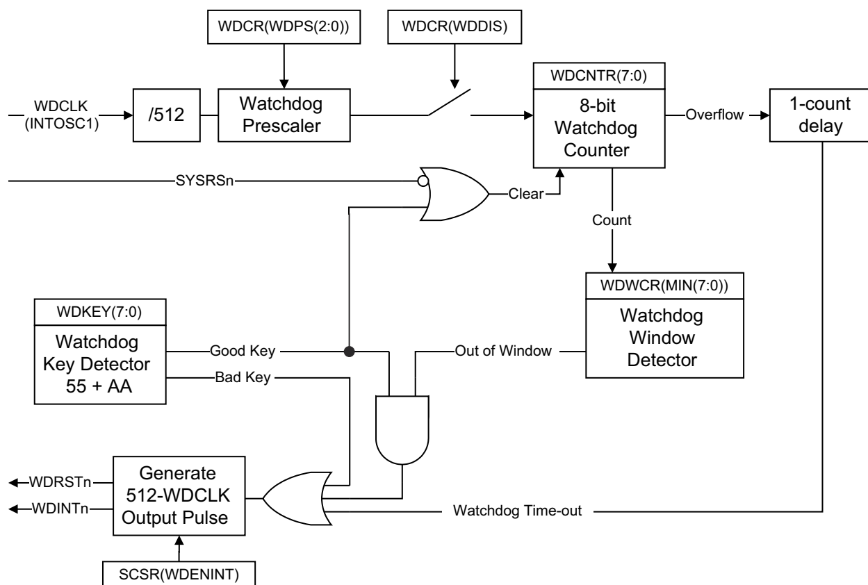
Figure 7-4. Windowed Watchdog
