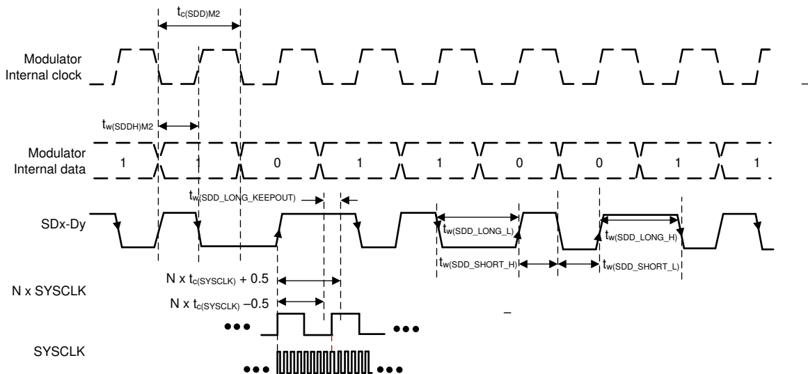
Figure 6-63. SDFM Timing Diagram – Mode 2
