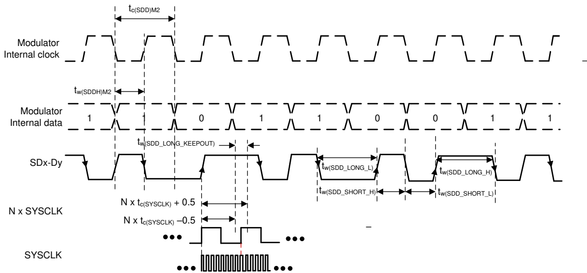
Figure 6-59. SDFM Timing Diagram – Mode 2
