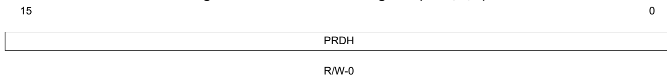
Figure 1-54. TIMERxPRDH Register (x = 0, 1, 2)
