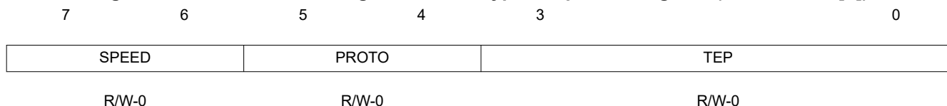
Figure 17-53. USB Host Configure Receive Type Endpoint n Register (USBRTYPE[ n ])
