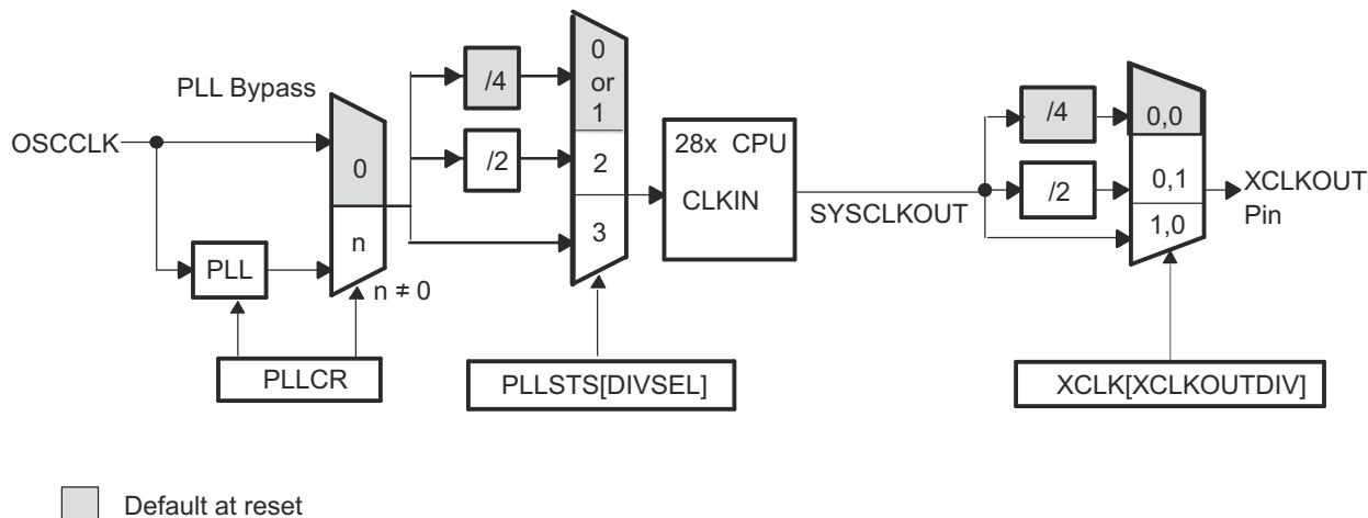
Figure 1-42. XCLKOUT Generation
