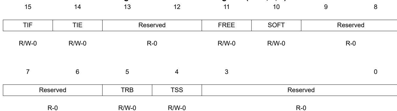
Figure 1-55. TIMERxTCR Register (x = 0, 1, 2)
