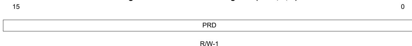
Figure 1-53. TIMERxPRD Register (x = 0, 1, 2)
