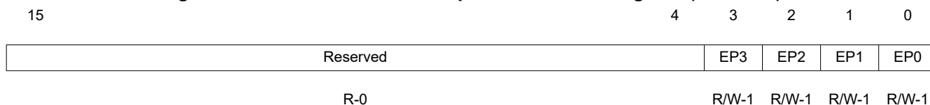
Figure 17-8. USB Transmit Interrupt Status Enable Register (USBTXIE)
