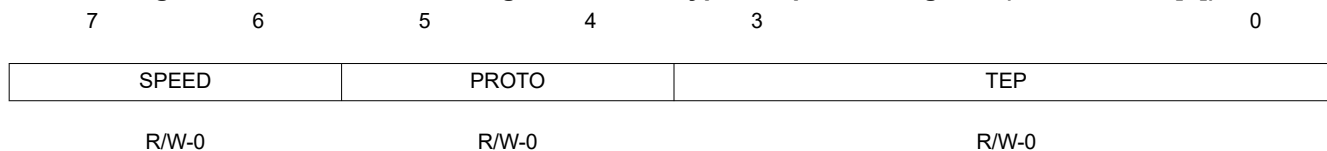
Figure 17-53. USB Host Configure Receive Type Endpoint n Register (USBRTYPE[ n ])
