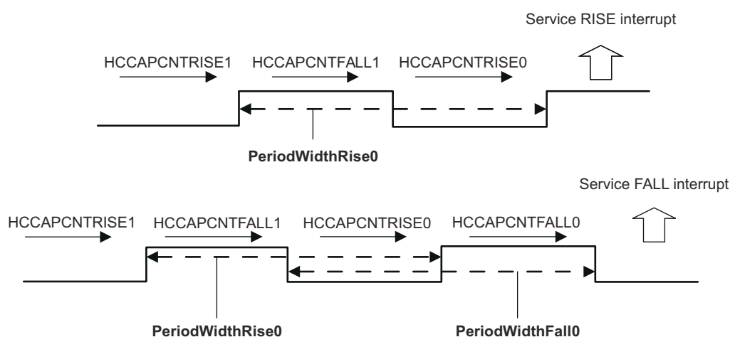
Figure 5-12. PeriodWidthRise0 and PeriodWidthFall0 Capture on RISE and FALL Events
