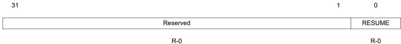
Figure 17-62. USB Device RESUME Raw Interrupt Status Register (USBDRRIS)
