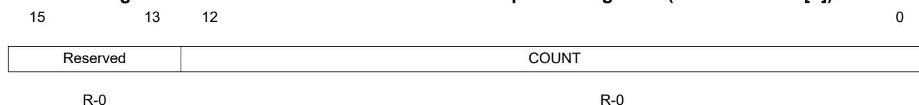
Figure 17-50. USB Maximum Receive Data Endpoint n Registers (USBXCOUNT[ n ])
