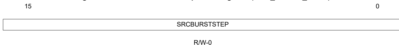
Figure 11-16. Source Burst Step Size Register (SRC_BURST_STEP)
