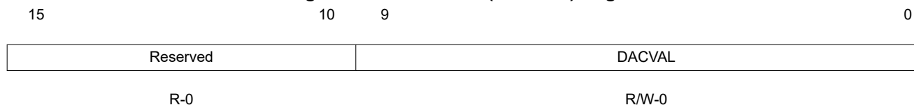
Figure 9-8. DAC Value (DACVAL) Register
