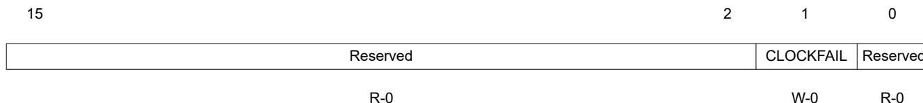
Figure 1-39. NMI Flag Force (NMIFLGFR) Register
